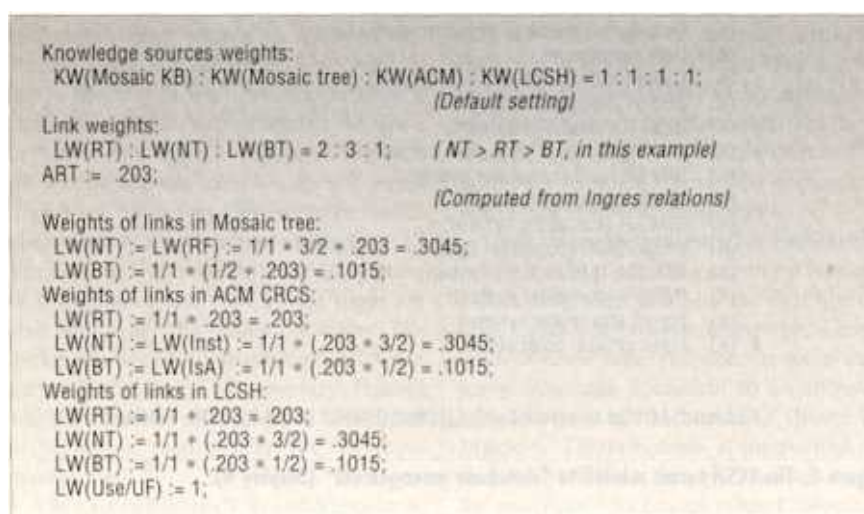
Figure 8. Link weights for the knowledge sources.
