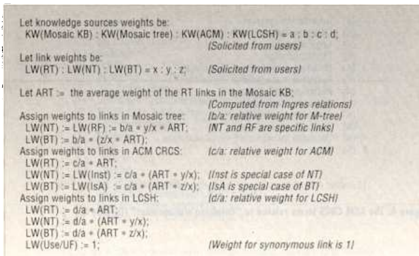
Figure 7. Connection weight assignments for the knowledge sources.
