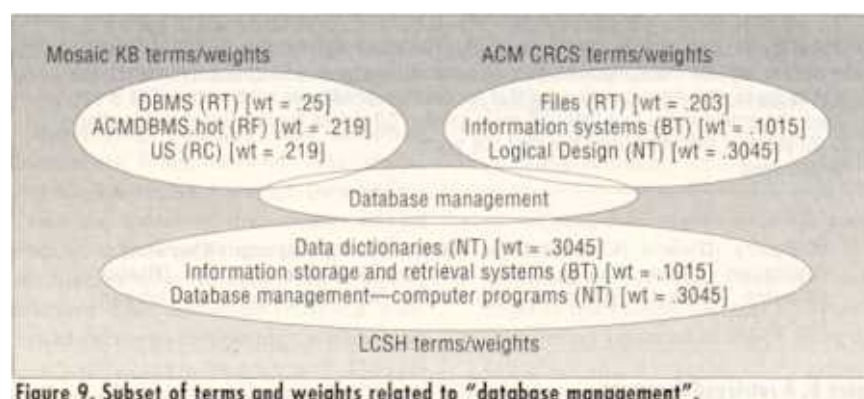
Figure 9. Subset of terms and weights related to "database management".
