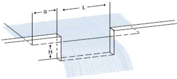
Figure 4. Diagram of a rectangular weir where L = width of weir opening (4 to 8 times H ), H = head of weir (measured 6 ft upstream of weir) and a = at least 3 \cdot H .
