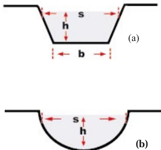
Figure 1. Cross-sectional dimensions for trapezoidal (a) and elliptical (b) ditches. (Diagram by J.S. Jones, 2003)
