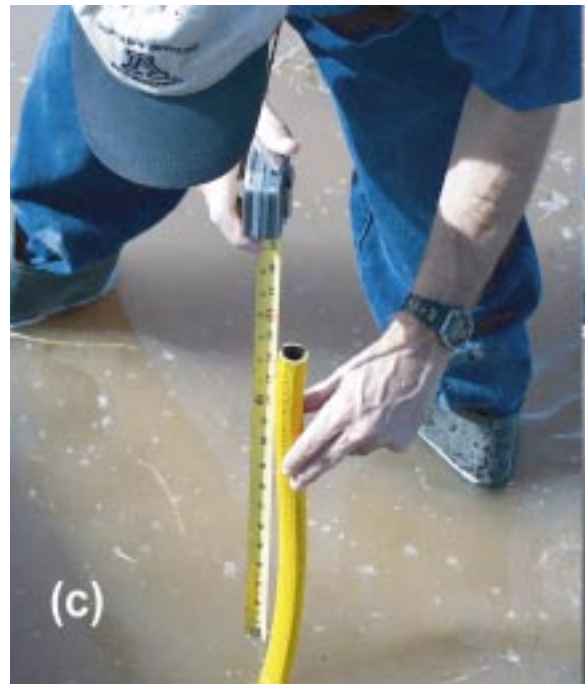
Figure 6. Three photos demonstrating how to measure the “drop” in a surface system. The drop is the distance from the level of the water in the ditch to the water level in the field. (a) Use the hose to siphon water out of the ditch; (b) Raise the hose up until water stops flowing out of the hose end; (c) Measure the distance between the end of the hose and the water level in the field.
