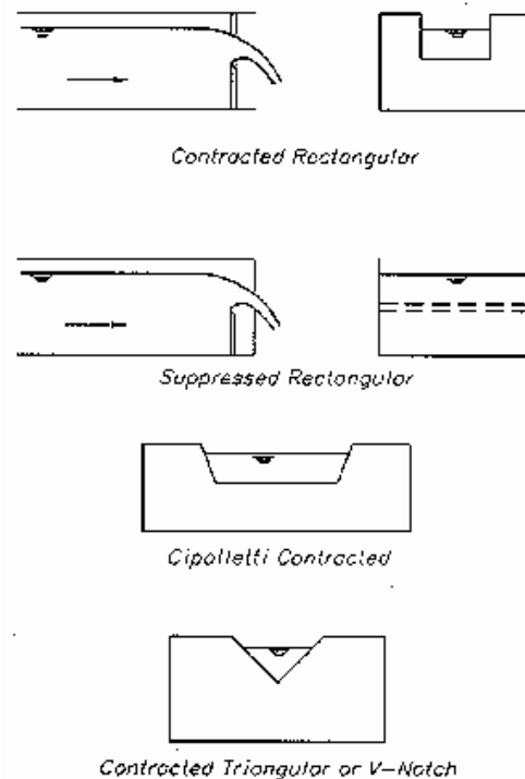
Figure 3. Diagrams of various types of weirs used to measure flow rate in an open ditch. (USDI-BOR, 1997).
