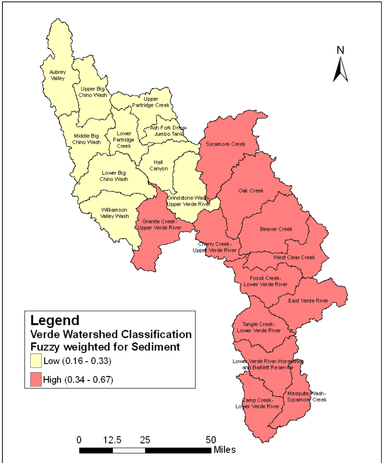
Figure 6-3: Results for the Fuzzy Logic Classification for Sediment Based on the Weighted Combination Approach.
