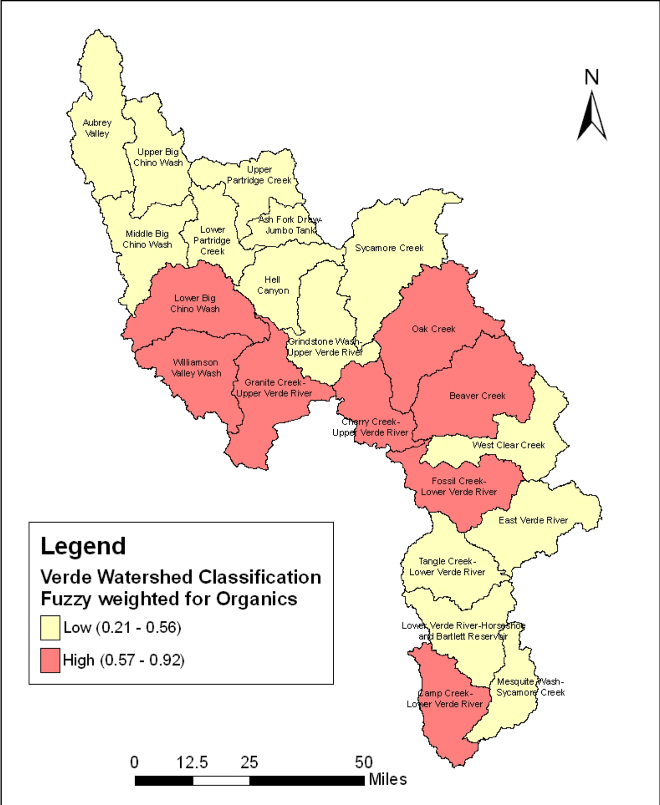
Figure 6-4: Results for the Fuzzy Logic Classification for Organics Based on the Weighted Combination Approach.
