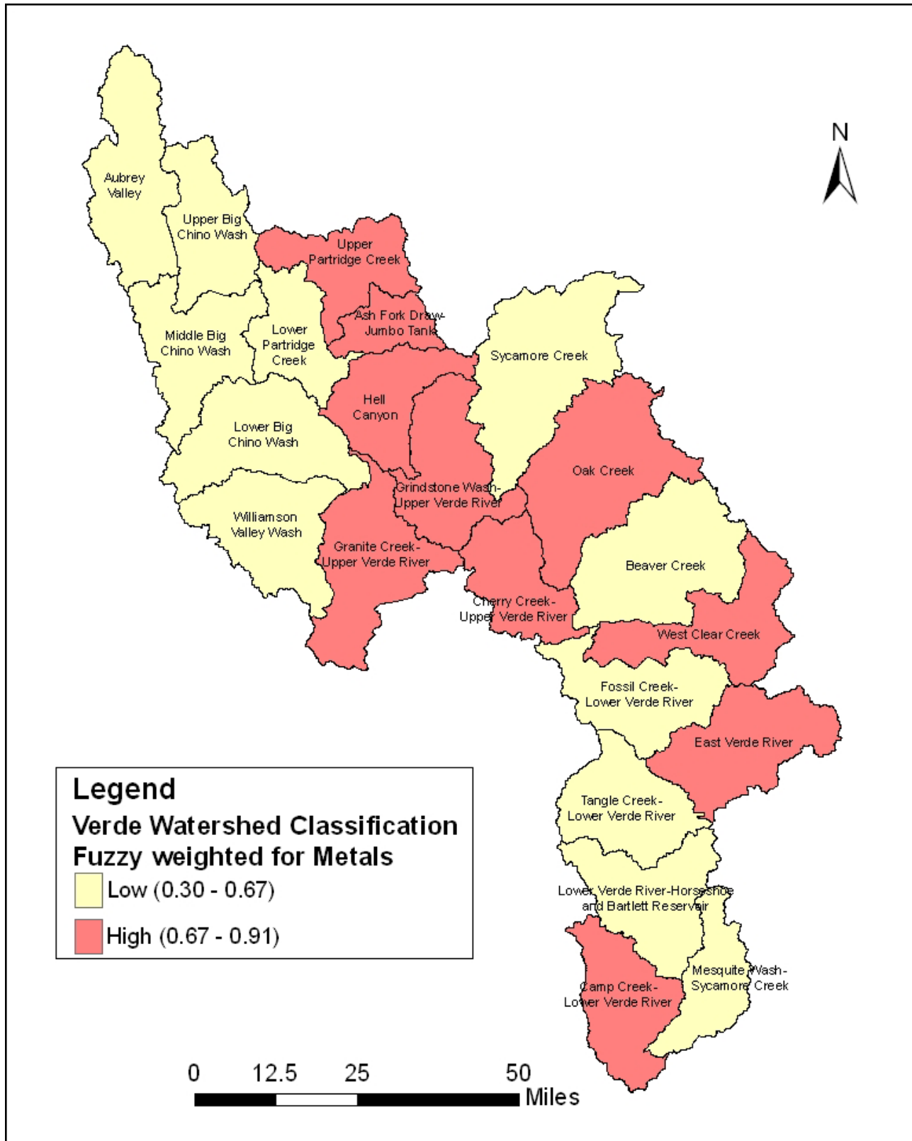
Figure 6-2: Results for the Fuzzy Logic Classification for Metals Based on the Weighted Combination Approach.
