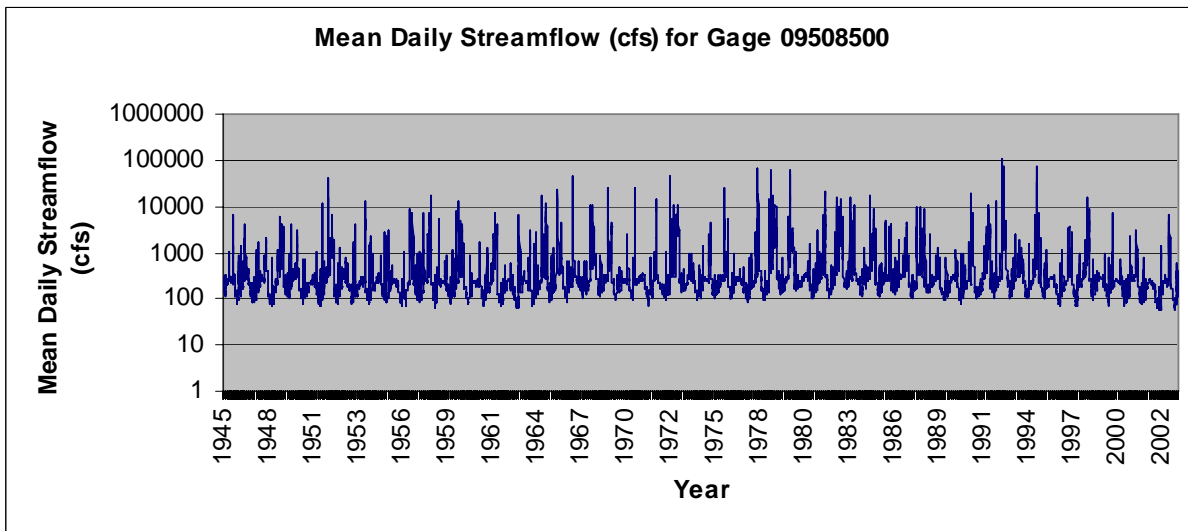
Figure 2-10: USGS Gage 09508500 (Verde River Below Tangle Creek, Above Horseshoe Dam) Hydrograph.
