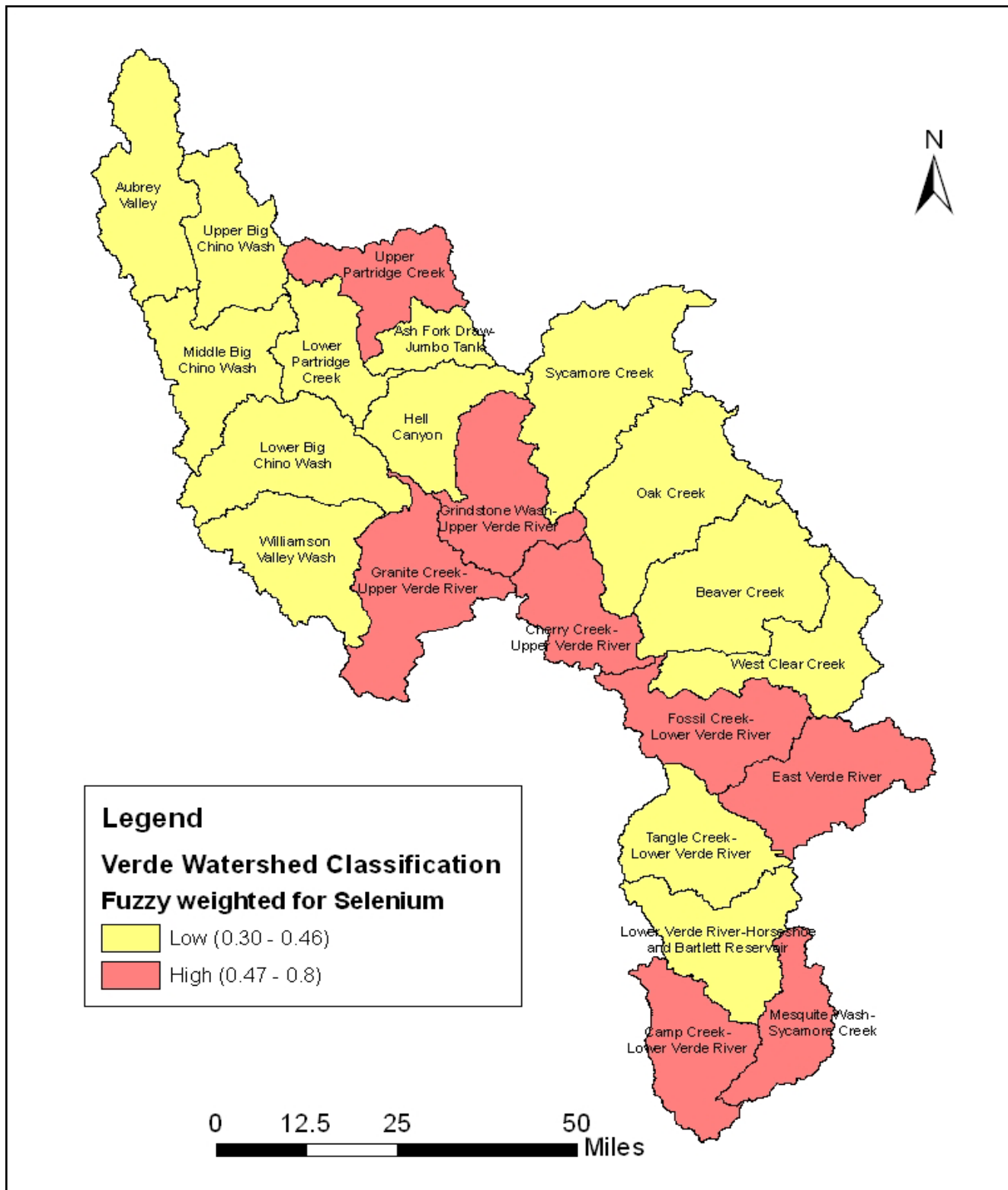
Figure 6-5: Results for the Fuzzy Logic Classification for Selenium Based on the Weighted Combination Approach.
