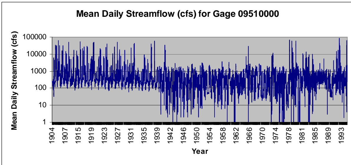
Figure 2-11: USGS Gage 09510000 (Verde River Below Bartlett Dam) Hydrograph.
