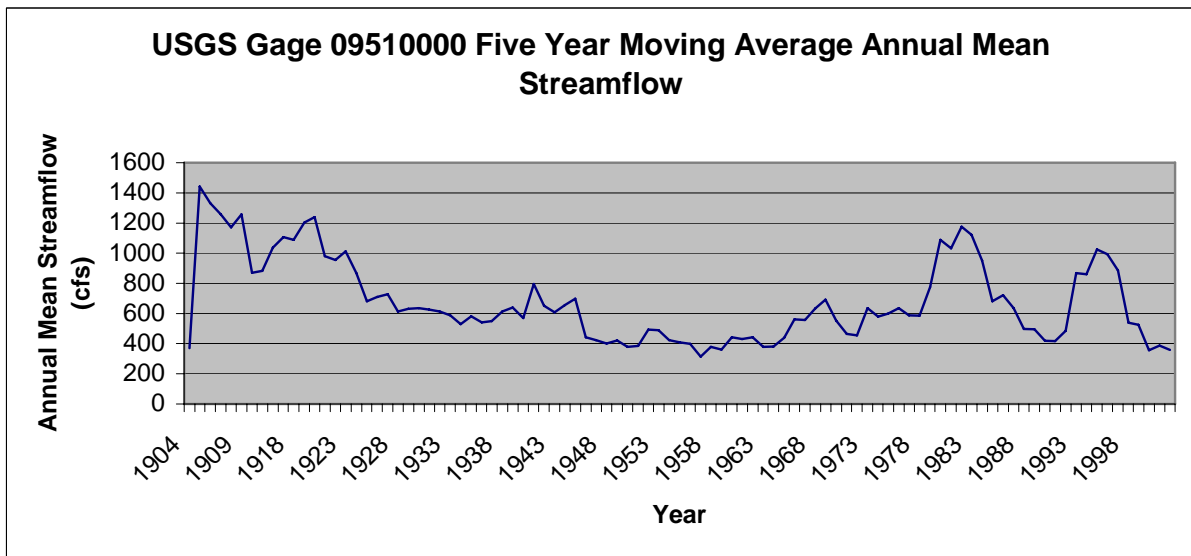
Figure 2-12: USGS Gage 09510000 (Verde River Below Bartlett Dam) Five Year Moving Average Stream Flow (cfs).
