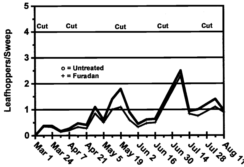
Figure 2b. 1999 leafhopper sweep net samples taken March 1 to August 11.
