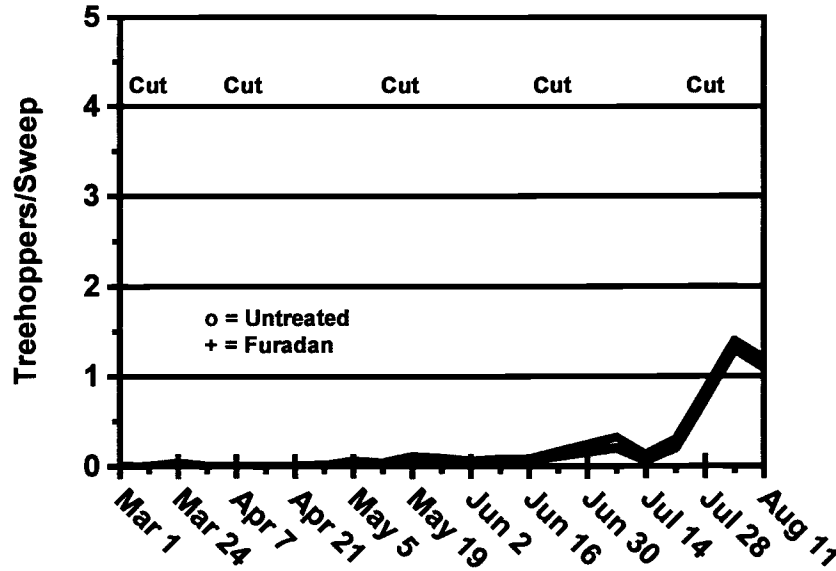
Figure 2a. 1999 treehopper sweep net samples taken March 1 to August 11.
