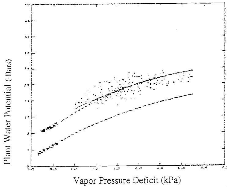
Figure 1. Plant Water Potential versus Air Vapor Pressure Deficit Transpiring at the Potential Rate (Idso, et. al)
