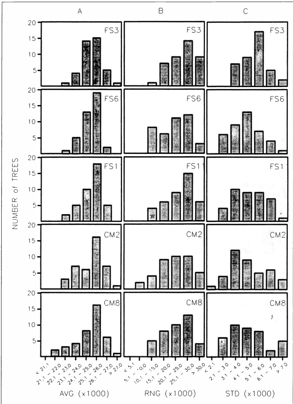
Figure 1. Number of trees classified by AVG (A), RNG (B), and STD (C) for five jack pine sites.
