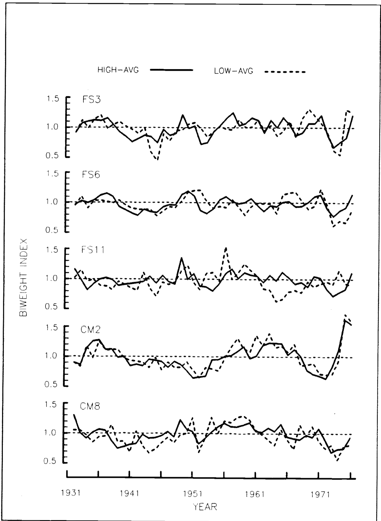
Figure 2. Biweight site chronologies for groups of high-AVG trees and low-AVG trees for five jack pine sites.
