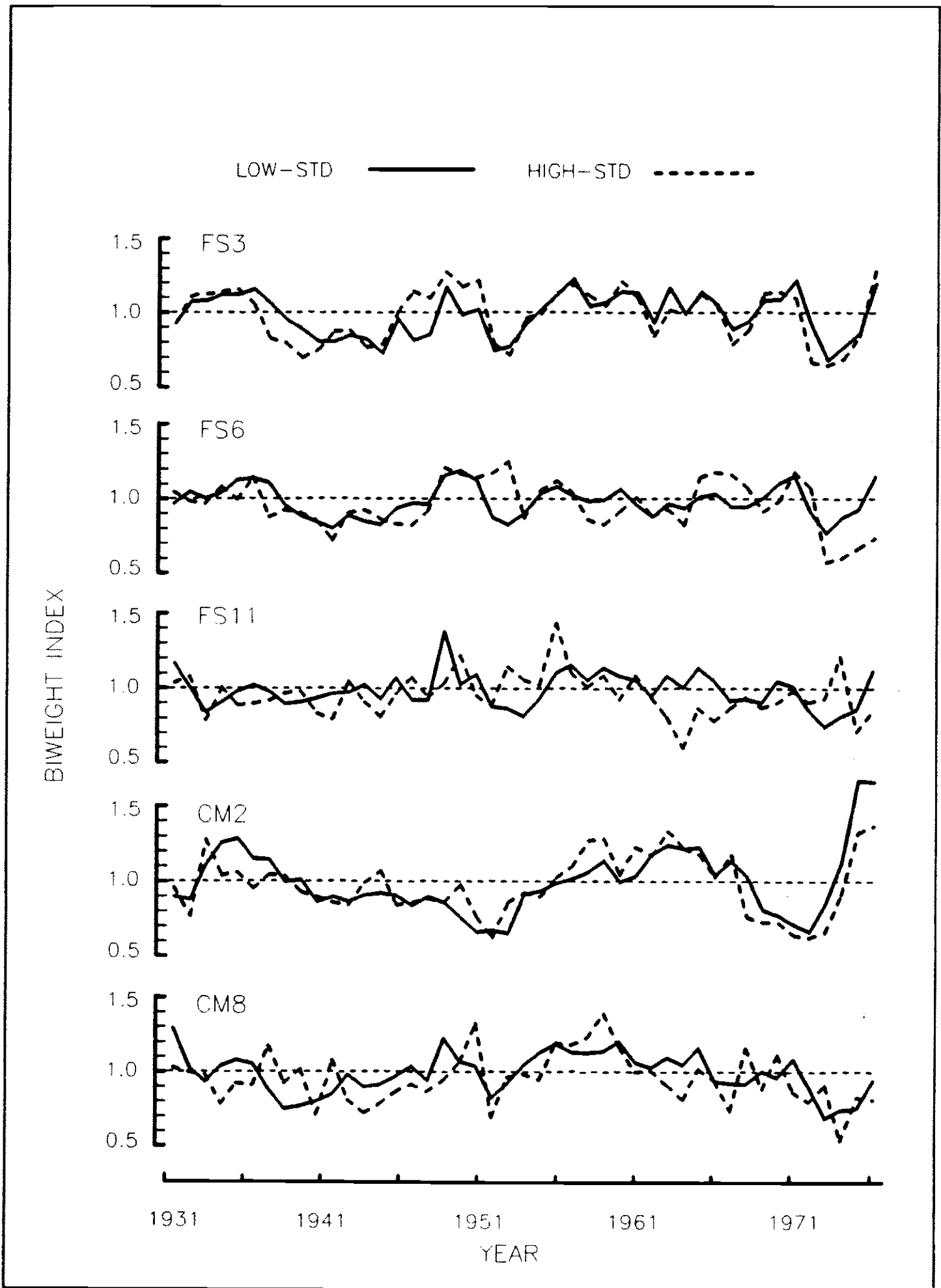
Figure 3. Biweight site chronologies for groups of high-STD trees and low-STD trees for five jack pine sites.
