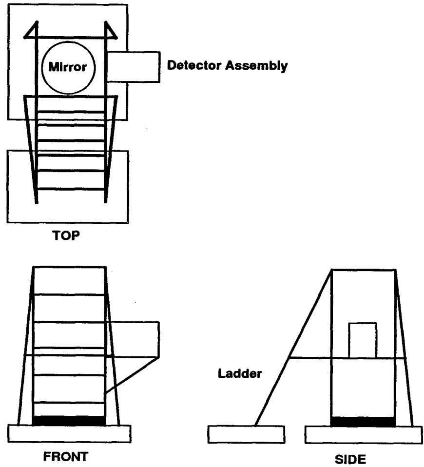
Figure 1.5 Diagram of Final Tower Design
