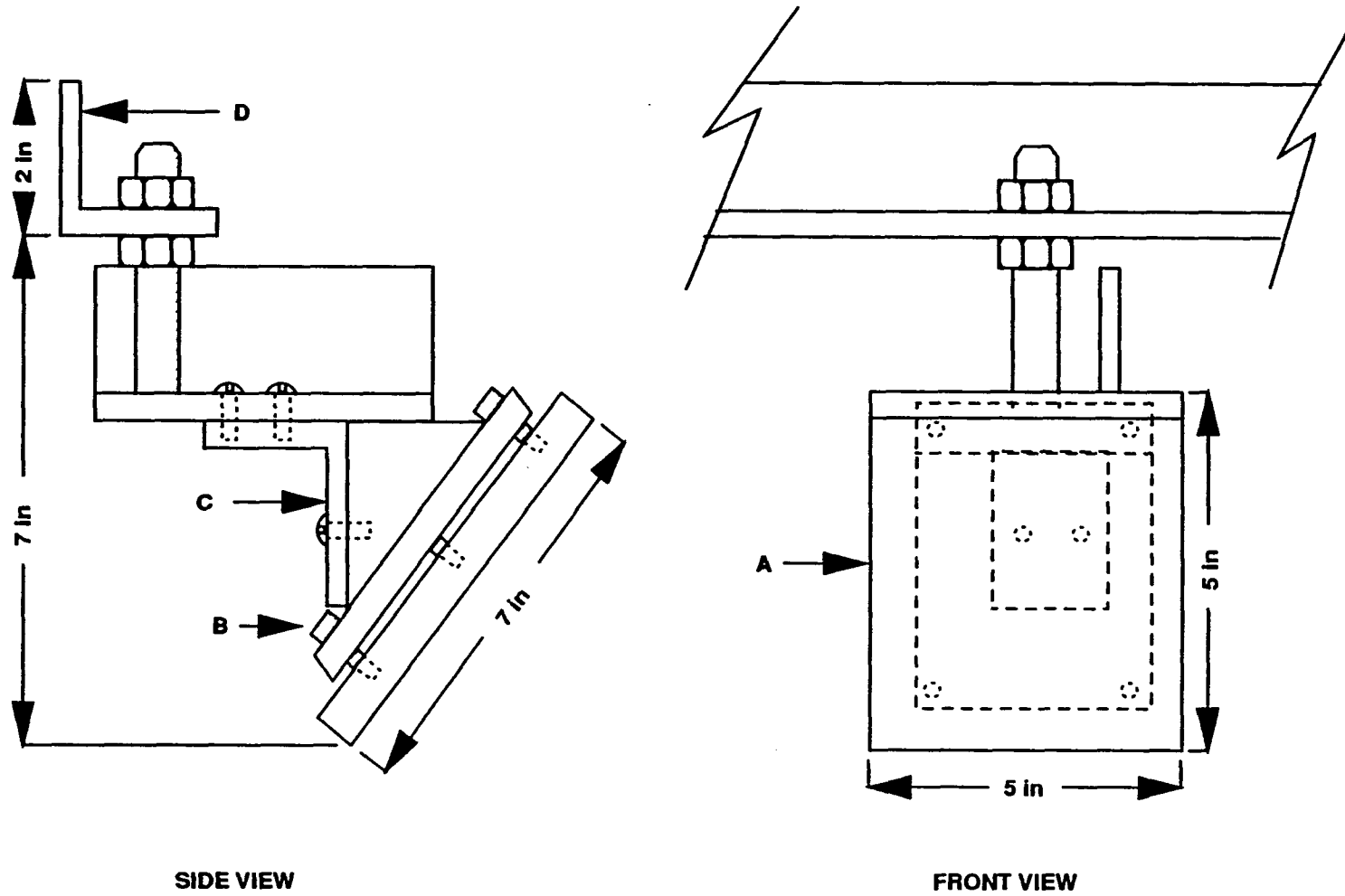
Figure 4.3 Secondary Mirror and Mounting Bracket
