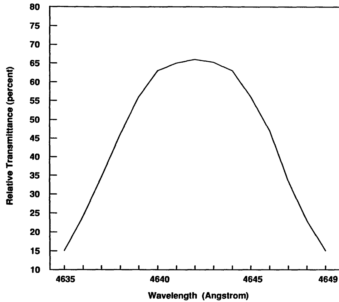
Figure 5.1 Bandpass Filter Transmittance Curve
