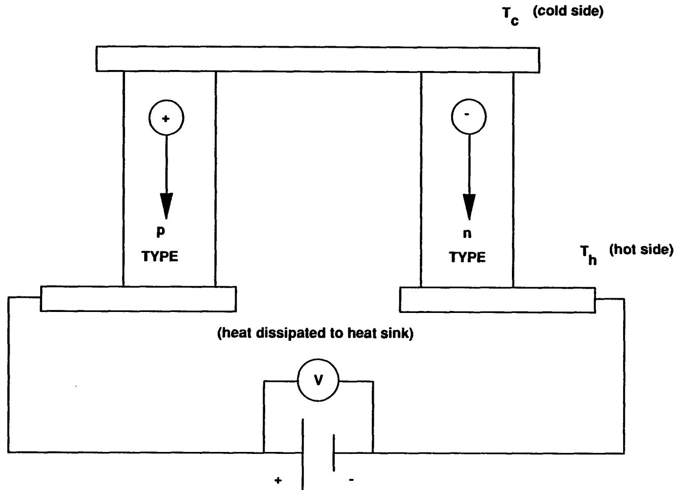
Figure 5.4 Diagram of a Thermoelectric Heat Pump
