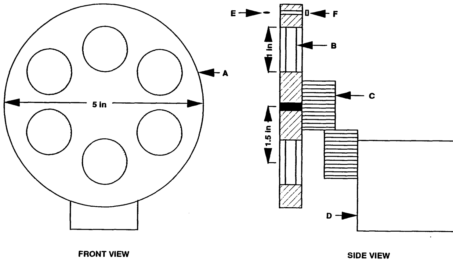
Figure 5.2 Bandpass Filter Wheel Assembly
