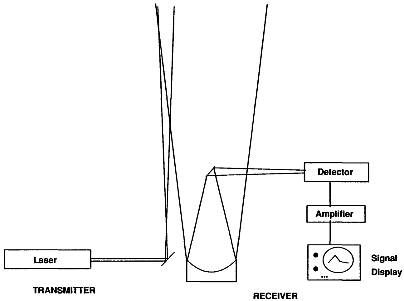
Figure 2.0 Biaxial Monostatic LIDAR System
