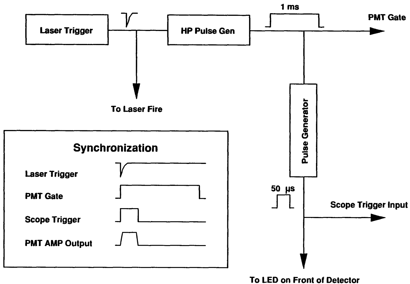
Figure 6.1 Control Electronics
