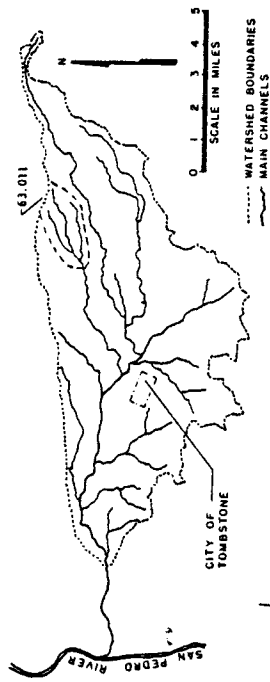
Figure 1. Location and map of Walnut Gulch watershed and subwatershed 63.011.
