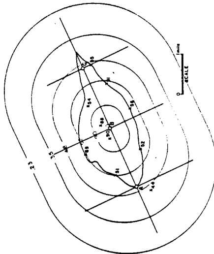
Figure 5. Model of simulated rainfall and orientation on watershed 63.011.
