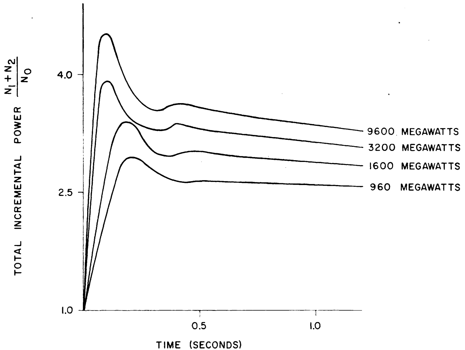
Fig. 7: Response of Linear System to a Step Demand in Power For Various Steady-State Power Levels, N_{oi}
