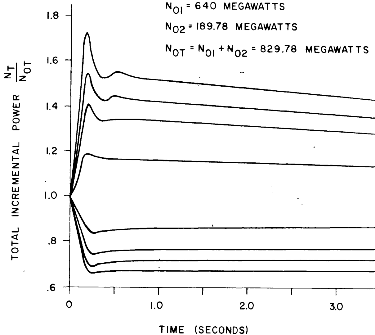
Fig. 10: Response of Coupled Core Reactor to a Step Demand in Power
