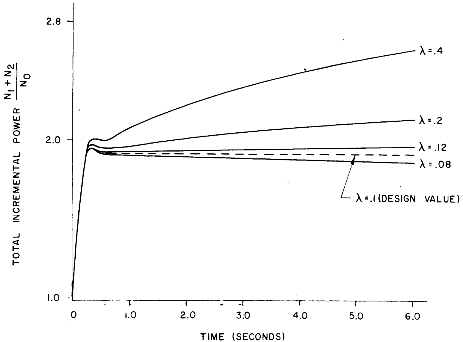
Fig. 5: Response of Linear System to a Step Demand in Power for Various Decay Constants, \lambda
