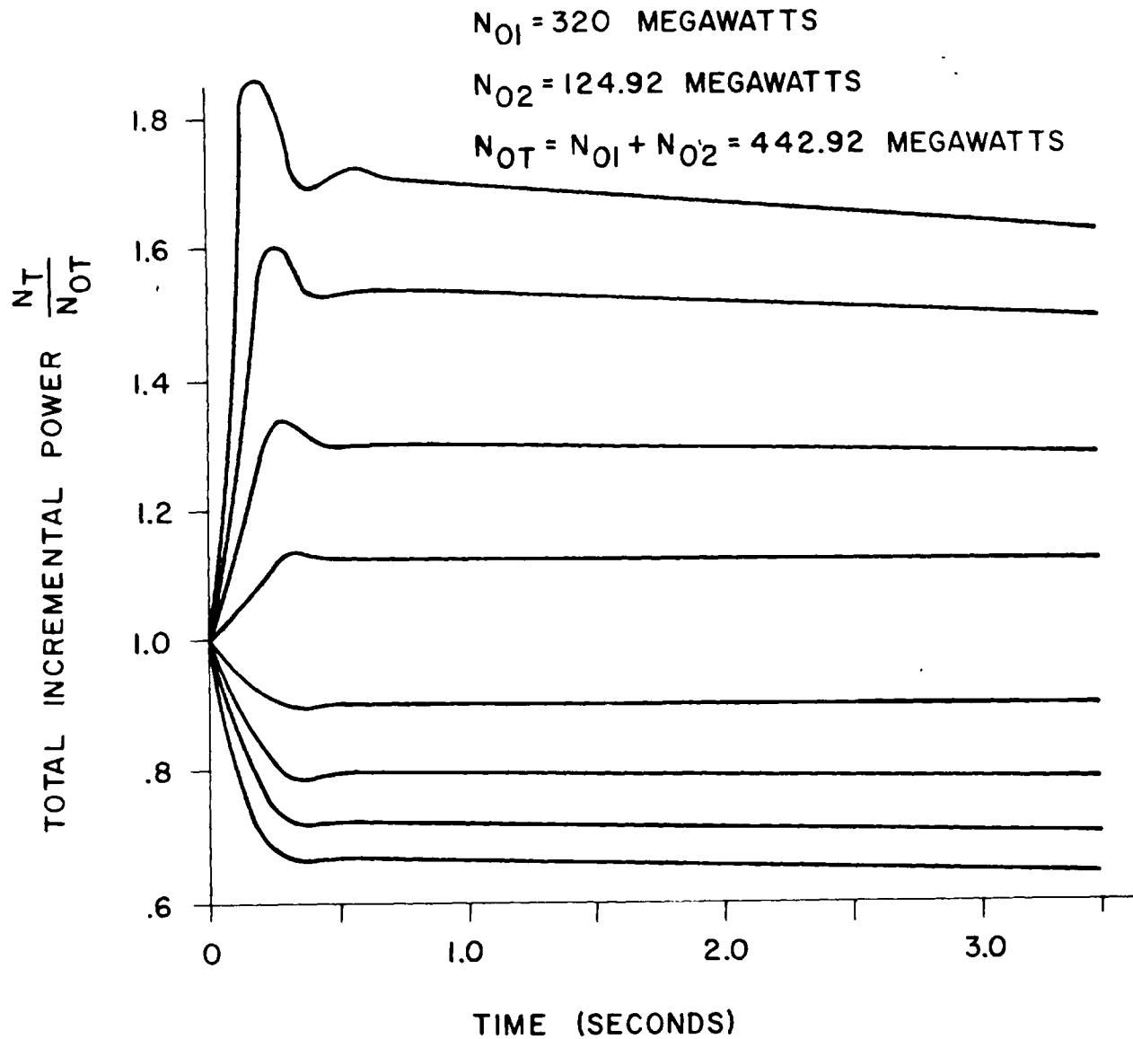
Fig. 9: Response of Coupled Core Reactor to a Step Demand in Power
