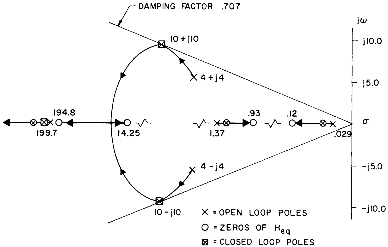
Fig. 6: Root Locus of Synthesized System
