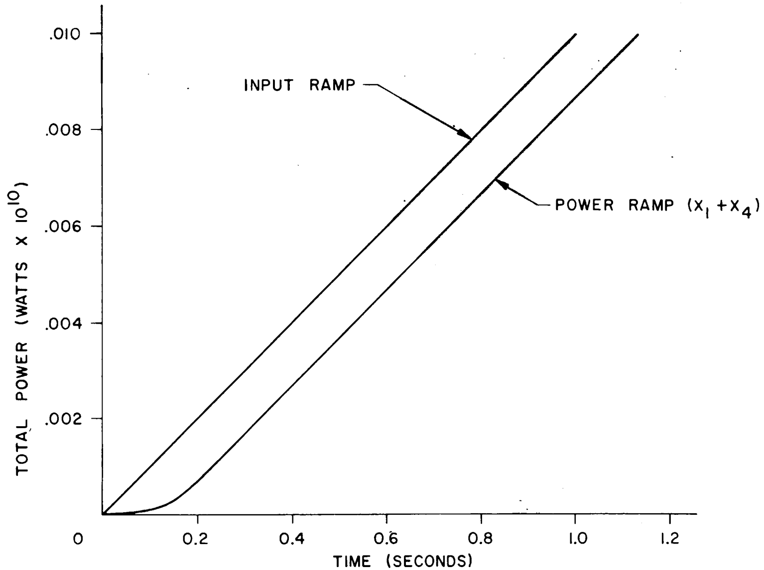
Fig. 8: Response of Linear System to a Ramp Demand in Power
