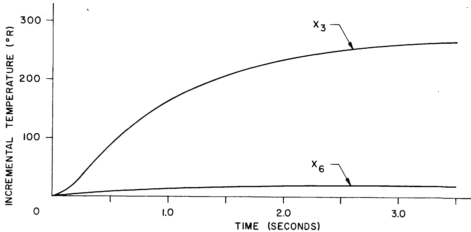
Fig. 3: Temperature Response to a Step Demand in Power
