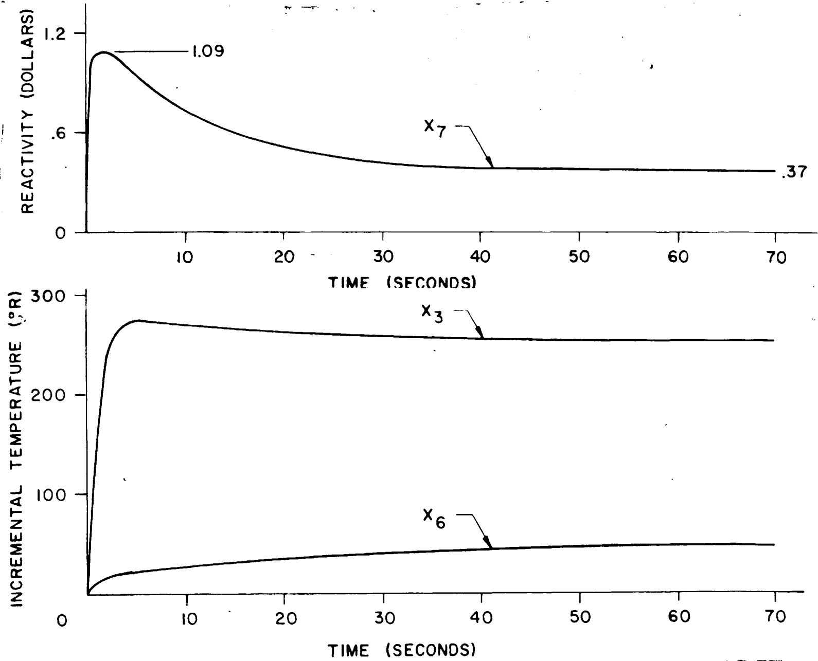
Fig. 2: State Variable Response of Linear System to a Step Demand in Power
