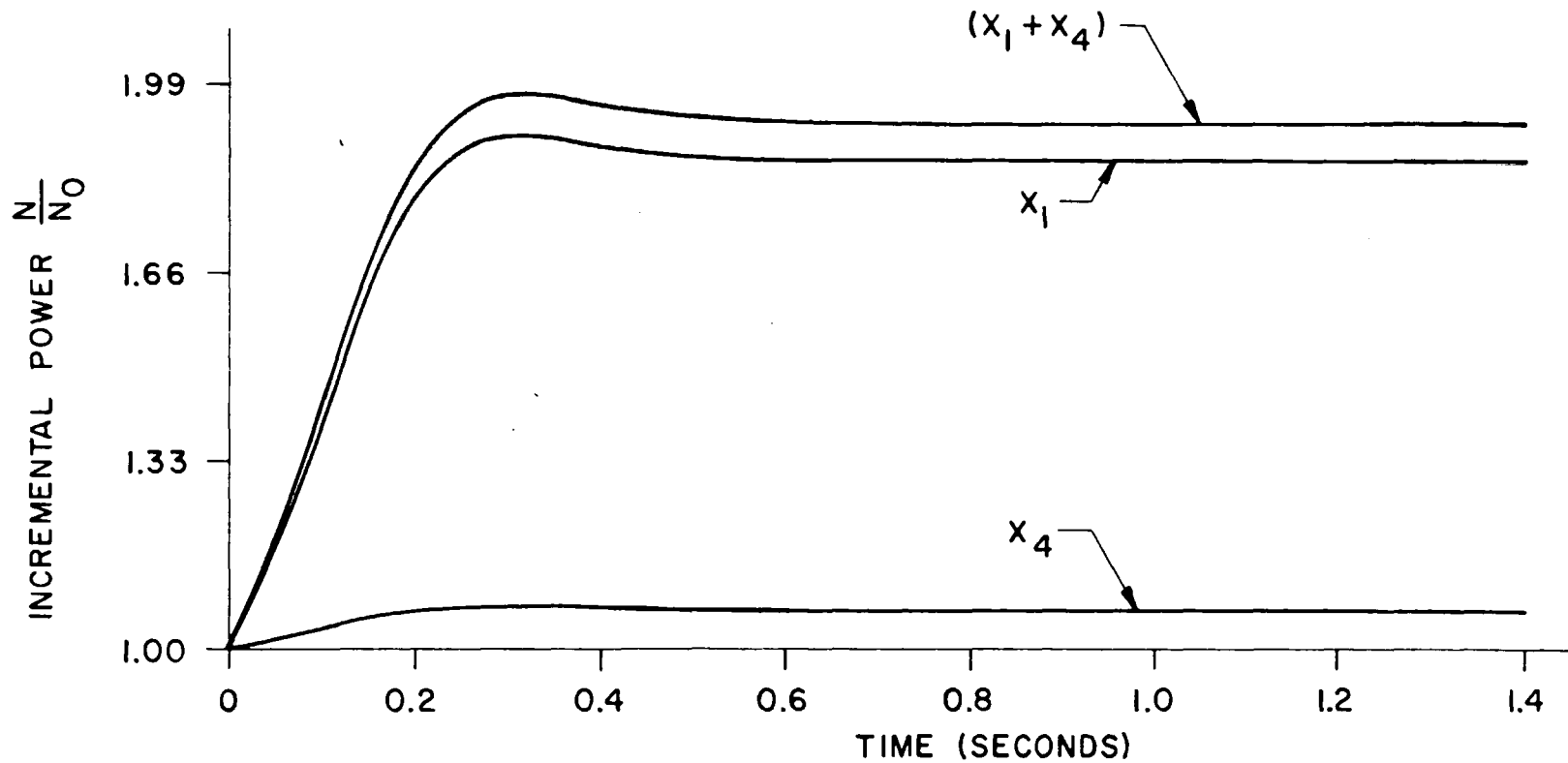
Fig. 1: Incremental Power Response of Linear System to a Step Demand in Power
