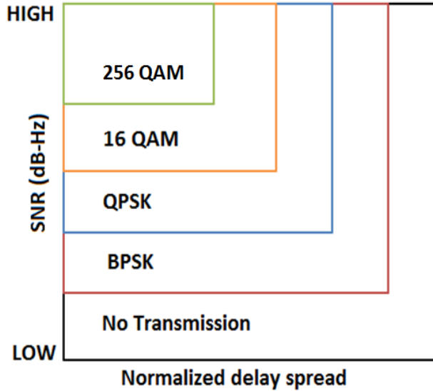
Figure 1: Link dependent adaptation
