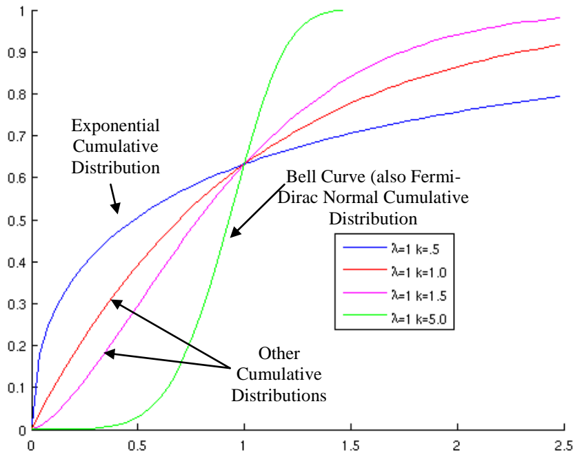
FIGURE 5 EXAMPLES OF CUMULATIVE DISTRIBUTION FUNCTIONS (INTEGRAL OF THE NORMAL DISTRIBUTIONS) FOR PROBABILITY DISTRIBUTION FUNCTIONS
