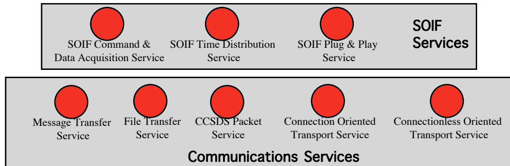
Figure 2 - User Applications View of SOIF Services
