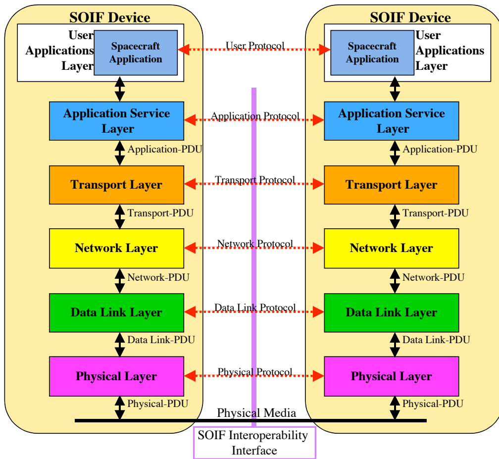
Figure 3 – Interoperability View of SOIF
