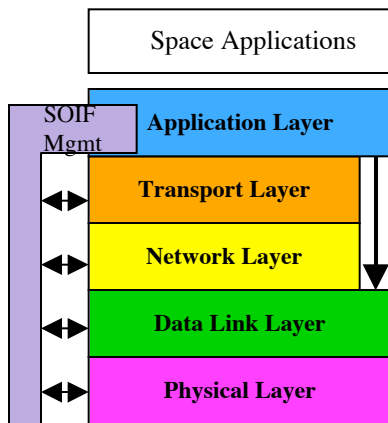
Figure 5 – Simplified SOIF Reference Model
