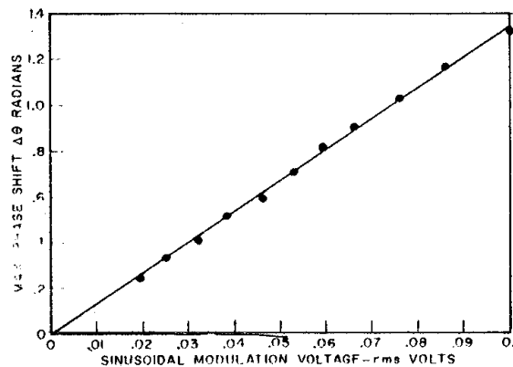
Fig. 4 - Modulation Sensitivity
