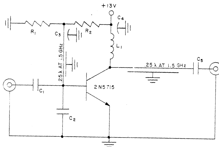
Fig. 8 - 1.5 Ghz Amplifier
