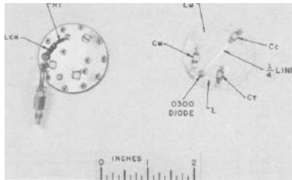
Fig. 6 - X20 S.R.D. Multiplier
