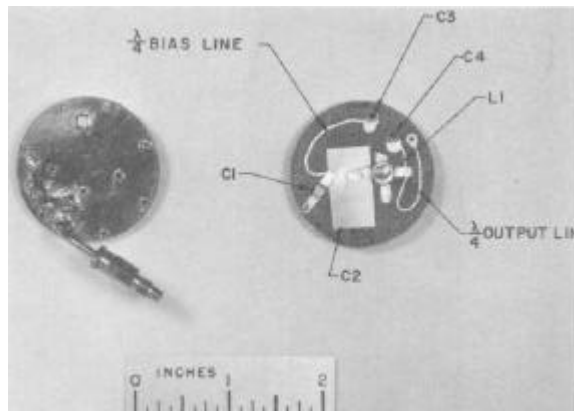
Fig. 8 - 1.5 Ghz Amplifier
