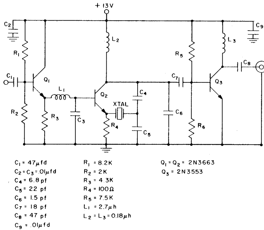
Fig. 2 - Modulator, 75-MHz Crystal Oscillator, and Power Amplifier
