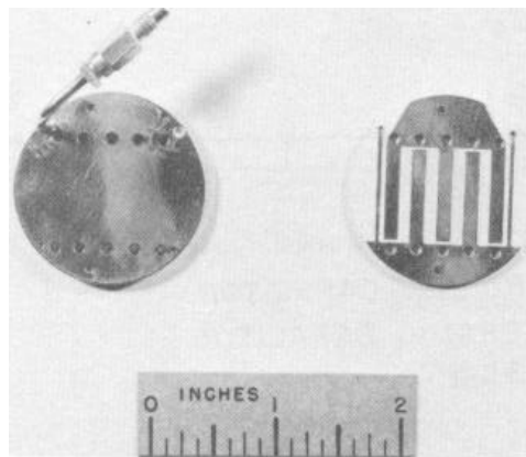
Fig. 7 - 1.5 GHz Interdigital Filter
