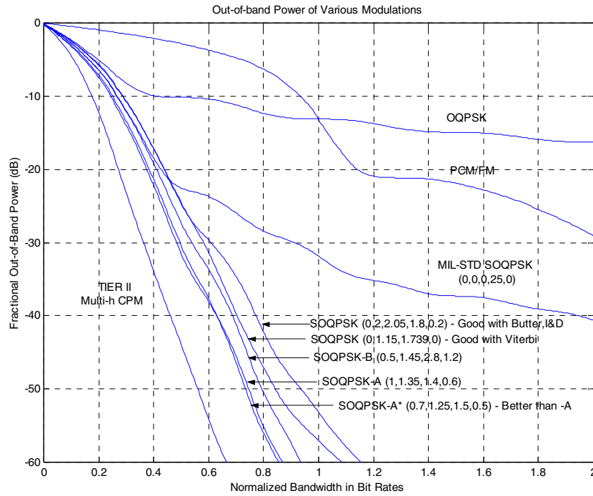
Figure 10. Fractional Out-of-Band Power of Various Modulations
