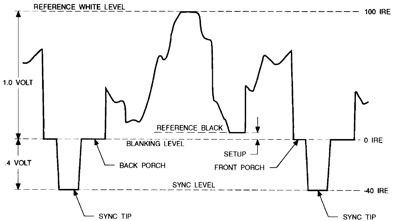
FIG. 1, MONOCHROME VIDEO WAVEFORM
