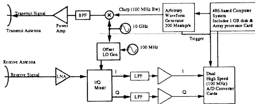
Figure 2: BYU SAR block diagram.
