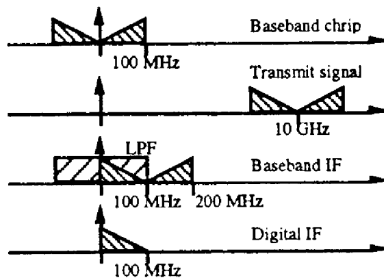
Figure 3: BYU SAR signal frequency plan.
