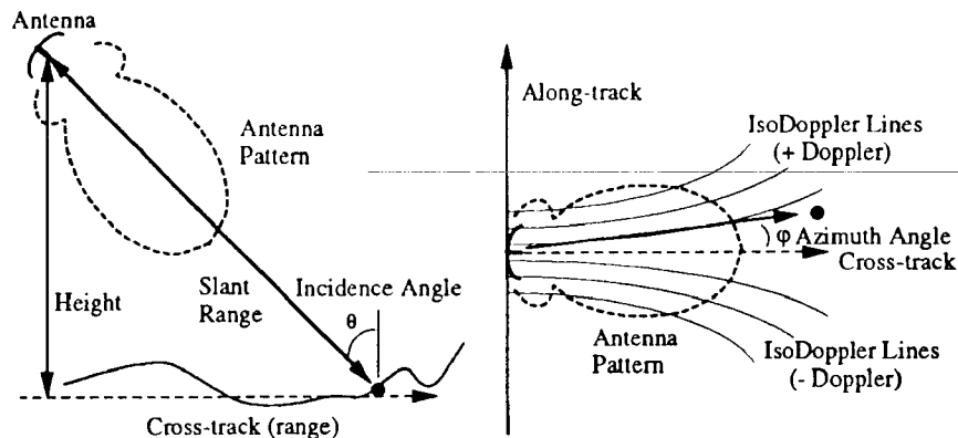
Figure 1: SAR observation geometry.
