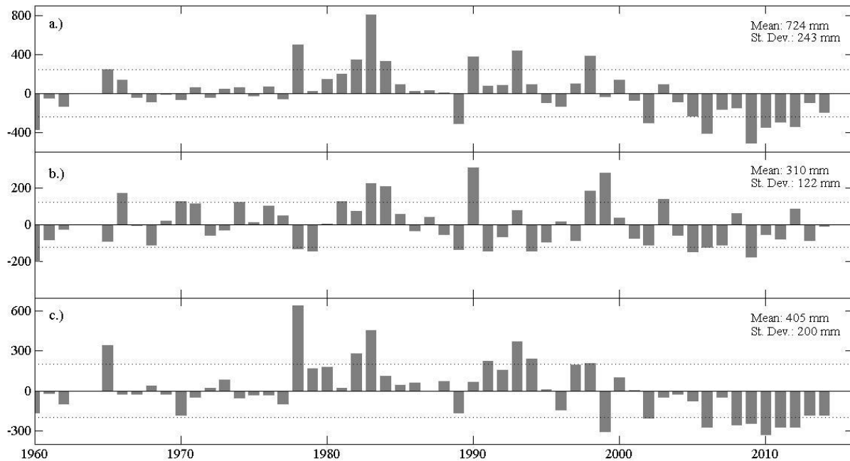
Figure 3. Long-term precipitation record from 1959 to 2014 at SCM-CZO for total annual (a.), summer (b.) and non-summer precipitation (c.) shown as anomaly or deviation from mean precipitation from 1959 to 2014. Dotted lines show standard deviation from mean precipitation over the entire record.
