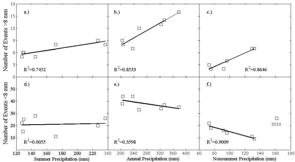
Figure 4. The relationship between total summer, annual, and non-summer precipitation for large events >8 mm (a.-c.) and small events <8 mm (d.-f.) at SRER-SRC. Year 2010 is considered an outlier and is excluded from linear analysis in non-summer precipitation for small events (f.).
