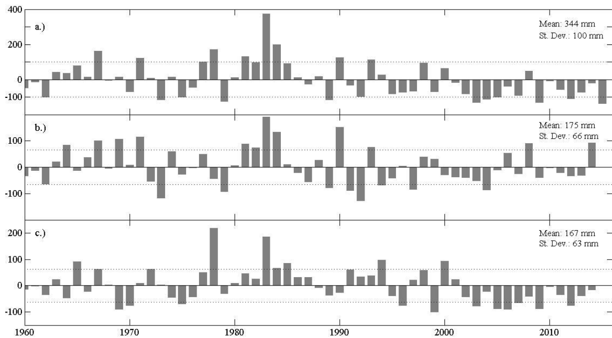
Figure 2. Long-term precipitation record from 1960 to 2015 at SRER-SRC for total annual (a.), summer (b.) and non-summer precipitation (c.) shown as anomaly or deviation from mean precipitation from 1960-2014. Dotted lines show standard deviation from mean precipitation over the entire record.
