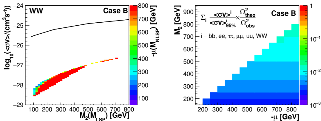
Figure 10. Case B: left panel shows the predicted cross section \langle\sigma v\rangle versus the DM mass (colored regions) and the limits from Fermi-LAT gamma-ray observation for the W^+W^- channel (the black curve). The color code indicates the \mu values. Right panel shows the normalized multiple channel cross section by the color code in the M_2 - \mu plane.
