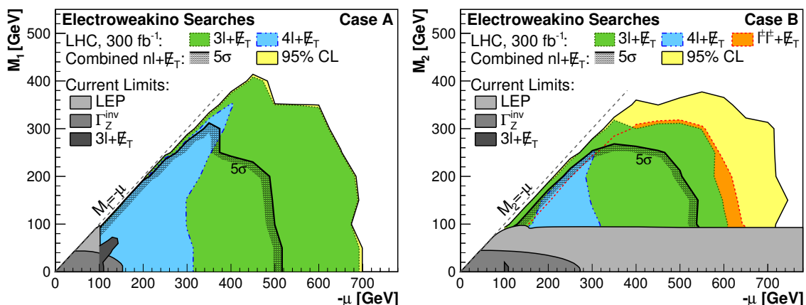
Figure 16. Estimated 95% CL. exclusion reach for electroweakino searches for Case A (left) and Case B (right). The colored regions show the same-sign di-lepton (orange), tri-lepton (green) and four-lepton (blue) channel as well as their combination (yellow). The combined 5\sigma discovery reach is indicated by the thick solid line next to the hatched region. Existing constraints from Electroweak Precision Measurements, LEP [50, 51] and LHC [60] are shown in gray shaded regions.
