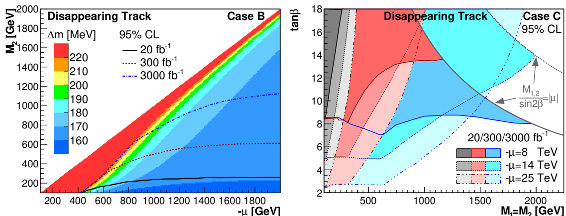
Figure 13. 95% CL exclusion from disappearing track searches at the LHC. Left panel for Case B in the M_2 - \mu plane: ATLAS at 8 TeV with 20 \text{fb}^{-1} (solid curve) and the projection for 14 TeV at 300 (dashed curve) and 3000 (dash-dotted curve) \text{fb}^{-1} , respectively. Mass difference \Delta m is shown by the corresponding color code. Right panel for Case C in the \tan\beta - M_{1,2} plane: ATLAS at 8 TeV with 20 \text{fb}^{-1} (far left black region) and the projection for 14 TeV at 300 (middle red region) and 3000 (right blue region) \text{fb}^{-1} , with three different values of \mu , respectively. The solid and dotted gray lines in the upper-right corner indicate the upper limit on M_{1,2} : M_{1,2}/\sin(2\beta) = |\mu| for a given value of |\mu| .
