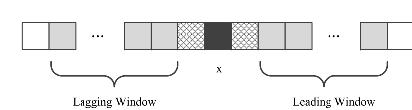
Figure 4: Adaptive threshold concept. x is the test sample, the hatched boxes are the guard samples, and the gray boxes are the sample used for the threshold calculation.
