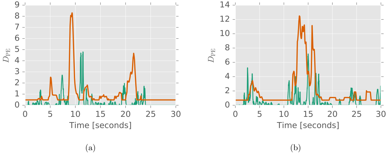
Figure 5: D_{PE} values (green curve) and threshold (orange curve) for a high- (a), low-risk individual (b). Candidate change points, \{t_{CP}\} occur when the green curve is greater than the orange curve.
