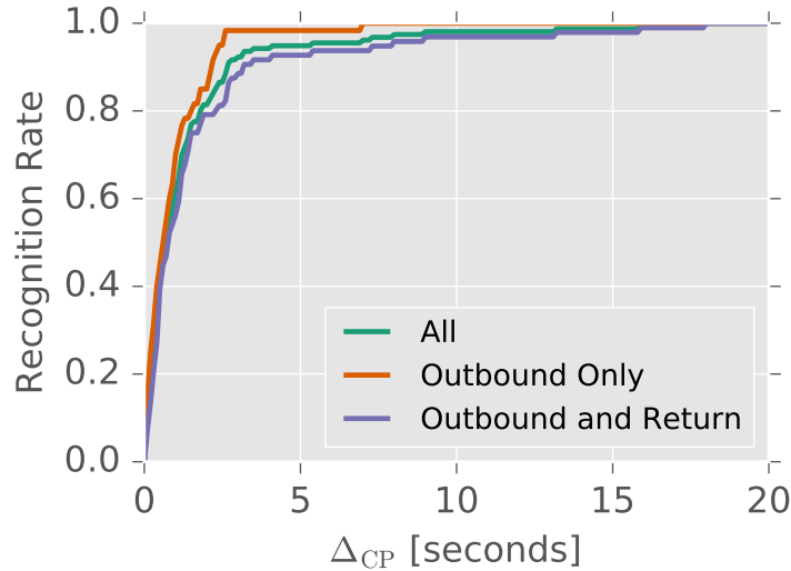
Figure 7: Detection rate versus difference between manually and algorithm identified change points \Delta_{cp} . For all gait segments, a recognition rate of 75% is achieved when \Delta_{CP} = 1.4 seconds
