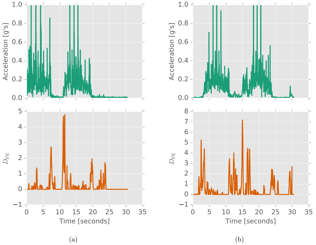
Figure 3: Dissimilarity measure or Pearson divergence D_{PE} for a high risk (a) and general risk faller(b). The top plots are the magnitude of the acceleration measurements, and the bottom plots are the D_{PE} .
