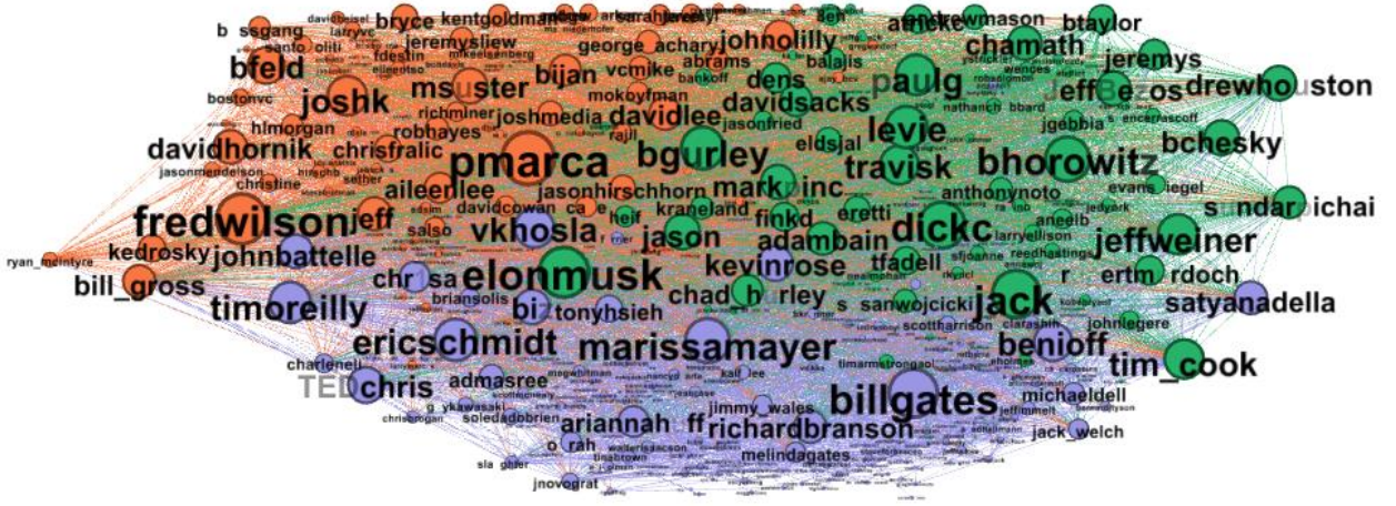
Figure 1 Network Graph
