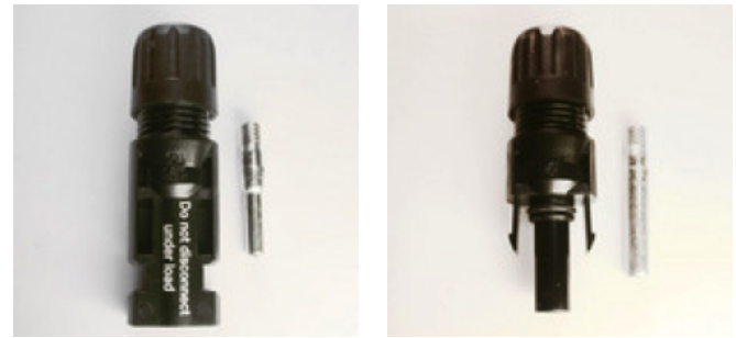
Figure 4. MC-4 multi contact connectors (male on left and female on right) are commonly found on commercial solar PV modules. The interlocking connectors prevent accidental disconnecting while under load. Source: PV-Cables, Inc.
