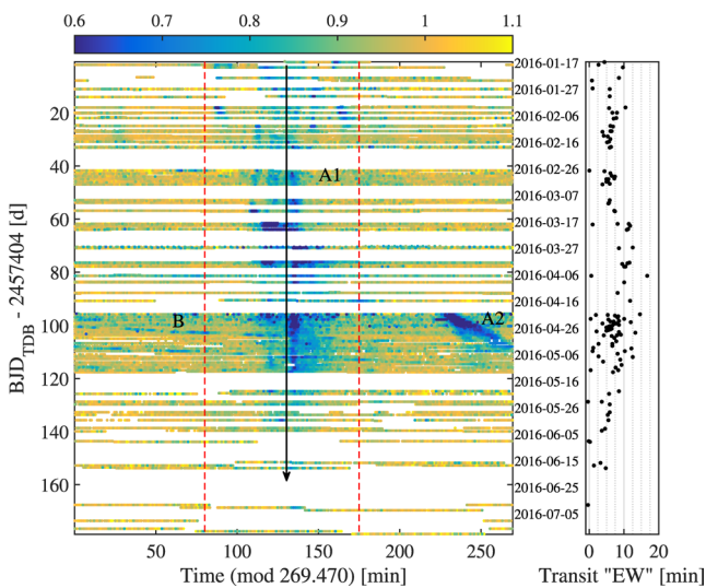
Figure B2. Left: ‘raw waterfall’ plot of the combined light curve, folded over the ‘A1’ period (269.470 min) and coloured by amplitude (from blue to yellow, with normalized flux ranging from 0.6 to 1.1). There are several dips sharing roughly the same period and lasting a few months. The black vertical arrow represents a constant period. Transits with different orbital periods (‘A2’ and ‘B’) appear as diagonal patterns. Right: transit ‘EW’. The dashed red lines on the left panel mark the EW integration limits.
