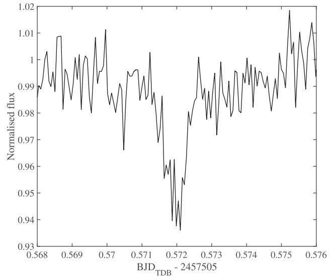
Figure B5. Part of our 2016 April 26 unbinned g' -band ULTRACAM light curve, showing an example of a smaller dip feature.
