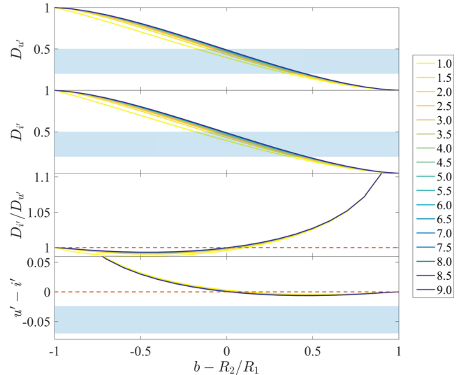
Figure 4. Limb-darkening simulation. From top to bottom: u' -band transit depth, i' -band transit depth, i' -band to u' -band transit depth ratio, and u' - i' -band colour index, as a function of the projected distance of the WD centre from the edge of the occulting disc at the time of mid-transit. The solid lines correspond to different R_2/R_1 values (see the legend). The blue-shaded areas in the top two plots mark the approximate observed transit depth range (20–50 per cent), while in the bottom plot it marks the 1\sigma - 3\sigma range of the colour detection ( -0.06 \leq u' - i' \leq -0.02 mag). The dashed red lines mark the bluing threshold ( D_{i'}/D_{u'} > 1 , u' - i' < 0 ). The maximal amount of bluing produced by limb darkening is much smaller than observed and its required transit configuration cannot explain the observed transit depths.
