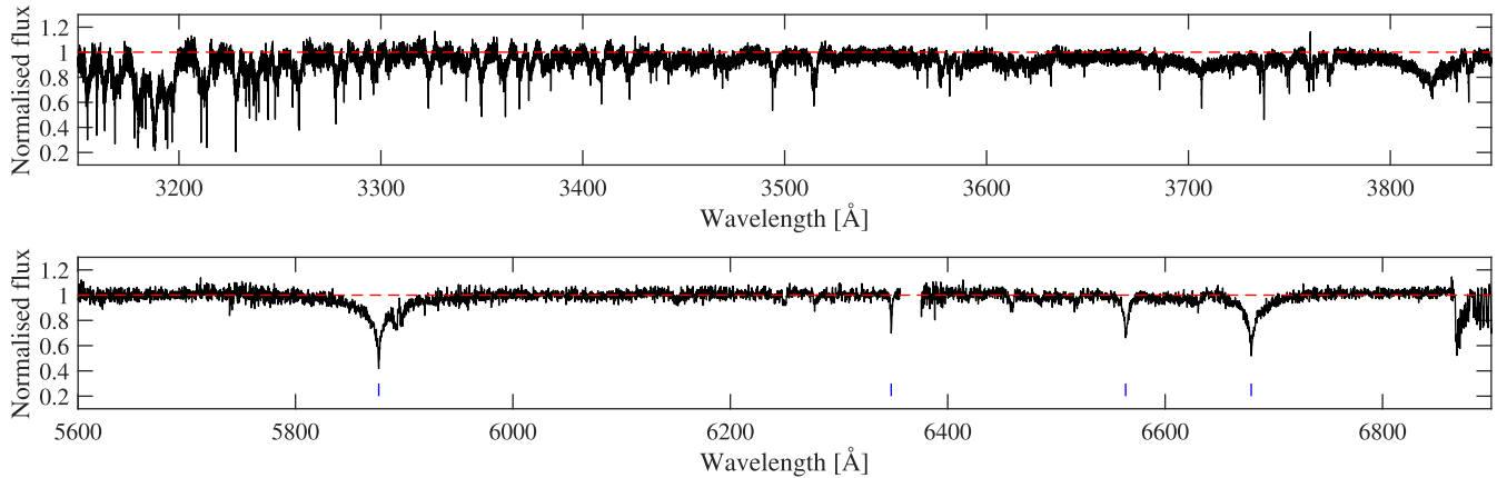
Figure 7. Top: normalized averaged Keck/HIRES spectrum from 2015 April 11 over the u' -band range (Xu et al. 2016). Note the increasing density of circumstellar absorption lines towards the ultraviolet side of the spectrum. Bottom: normalized averaged VLT/X-SHOOTER spectrum from 2016 March 29, over the r' -band range. The blue ticks mark the photospheric absorption lines (other features are telluric).
