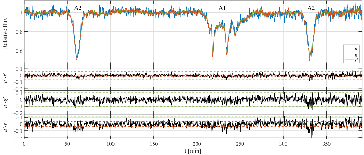
Figure 1. Top: ULTRACAM light curve from 2016 April 21, in u' (blue), g' (green) and r' (red) bands, binned to an effective exposure time of 20 s. The labels above the dips denote dips which share a common period. Bottom: colour indices, as marked (black solid line). The dashed lines indicate the 1\sigma (red) and 3\sigma (green) levels. Note the 2-3\sigma detection of bluing during transits only, as evidenced by negative values of u' - g' and u' - r' .
