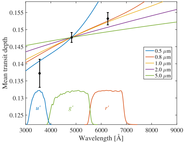
Figure 5. The mean transit depth in u' , g' and r' bands (black error bars) for the first ‘A2’ dip in the ULTRACAM light curve from 2016 April 21. The filter bandpasses are shown below each error bar. The coloured curves correspond to the extinction cross-section curves of ‘astronomical silicate’ for various effective grain radii (see the legend), all scaled to fit the g' -band measurement. The curves for \sim 0.8 – 2 \mu\text{m} -sized grains can match the observed bluing, but rather marginally.
