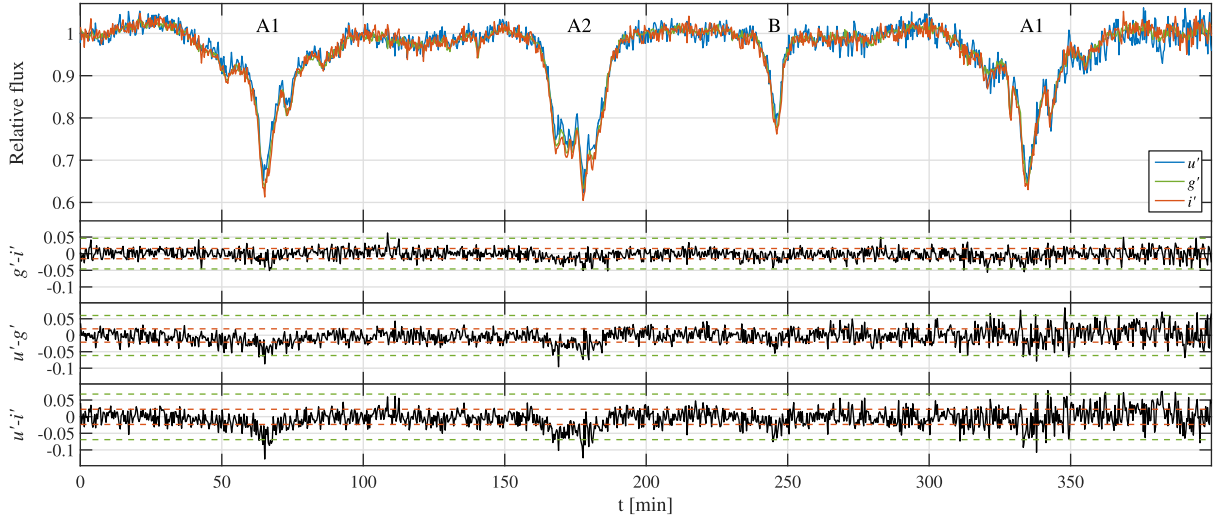
Figure 2. Same as Fig. 1, for 2016 April 26, with i' band instead of r' band. Note the significant evolution of the light curve in merely five nights: the change in the shape of the ‘A1’ and ‘A2’ dips, and the appearance of the ‘B’-dip (see Appendix B).
