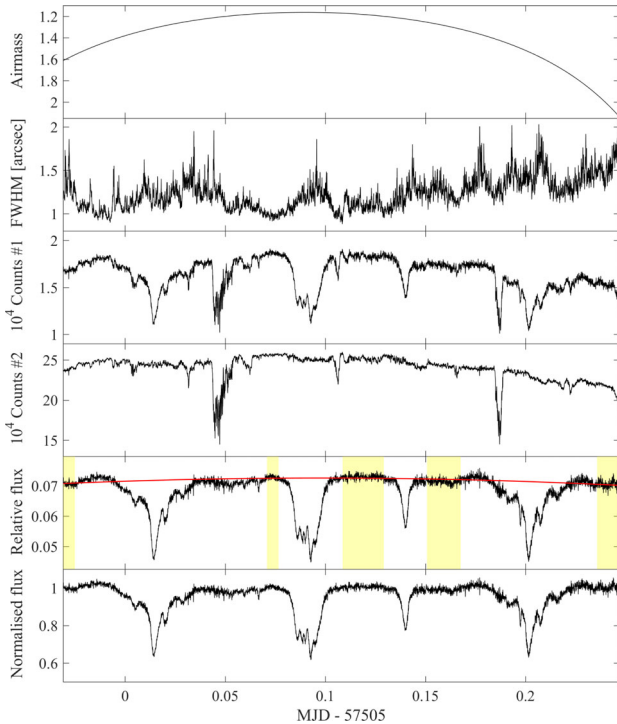
Figure A2. Same as Fig. A1, for 2016 April 26. Note the sharply falling atmospheric transmission at several times (generally outside of transits, e.g. at MJDs \sim 57505.05 , 57505.11 and 57505.19 ), indicating passing clouds.
