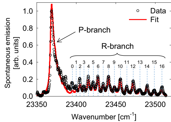
FIG. 2. Experimental data and a fit for spontaneous emission detected from the side, in the case of pumping 4 torr of pure nitrogen with 2 mJ, 60 fs laser pulses at 1500 nm wavelength. The tabulated values of the wave number for different rotational transitions [14] are marked with vertical dashed lines. The corresponding values of the rotational quantum number N'' in the lower emission state are shown next to the individual lines. Spontaneous emission peaks at N'' = 6 .
