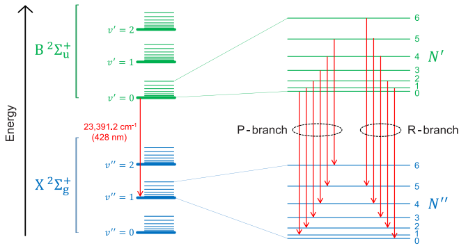
FIG. 1. Left: A diagram of the B^2\Sigma_u^+ and X^2\Sigma_g^+ electronic energy manifolds of the N_2^+ molecular ion. Integers v' and v'' index different vibrational levels within the upper and lower electronic manifolds, respectively. Right: An expanded diagram of vibrational energy manifolds v' = 0 and v'' = 1 within the upper and lower electronic energy manifolds. N' and N'' are the nuclear-angular-momentum quantum numbers in the upper and lower emission states, respectively. In this Rapid Communication, different spectral lines within P and R emission branches are numbered by the quantum number N'' of the lower rotational state involved in the particular transition.
