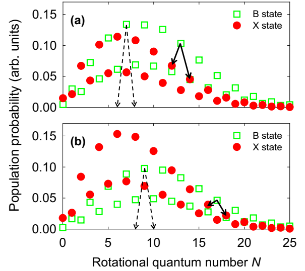
FIG. 4. (a) Rotational population distributions in the upper and lower emission levels of the N_2^+ molecular ion, inferred from fitting of the experimental data. Allowed transitions that produce the strongest spontaneous and stimulated emissions are marked with dashed and solid arrows, respectively. (b) Rotational distributions calculated according to Eqs. (1) and (2) with N_B = 5 and N_X = 0 and negative net electronic population inversion [the ratio of total populations in the B^2\Sigma_u^+(0) and X^2\Sigma_g^+(1) states equals 0.75]. Population inversion and gain still exist on a subset of rotational transitions with large values of the rotational quantum number N .
