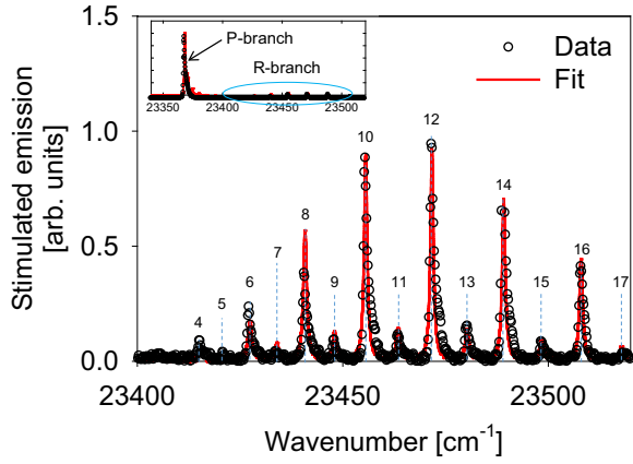
FIG. 3. Same as in Fig. 2, but for the stimulated emission that is self-seeded by the spectrally broadened third harmonic of the pump and measured in the forward direction. The R-branch emission, which comprises the transitions with the change of the nuclear-angular-momentum quantum number N of -1 , is shown in the main figure. The inset shows the full emission spectrum including both P- and R-branch emissions. Stimulated emission peaks at the N'' value of 12, which is larger than the peak value for spontaneous emission. Based on the ratio of the stimulated-emission signals on the adjacent spectral lines in the R branch, we estimate the peak value of the total gain in the 1-mm-long interaction zone as 64, corresponding to the lower-bound estimate for the peak exponential gain per unit length on the strongest R-branch line of about 40 \text{ cm}^{-1} .
