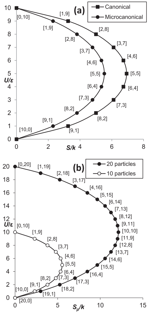
FIG. 1. (a) Internal energy–entropy profiles for N = 10 PSL under microcanonical and canonical conditions. (b) Internal energy–entropy profiles for microcanonical PSLs with N = 10 and N = 20 .
