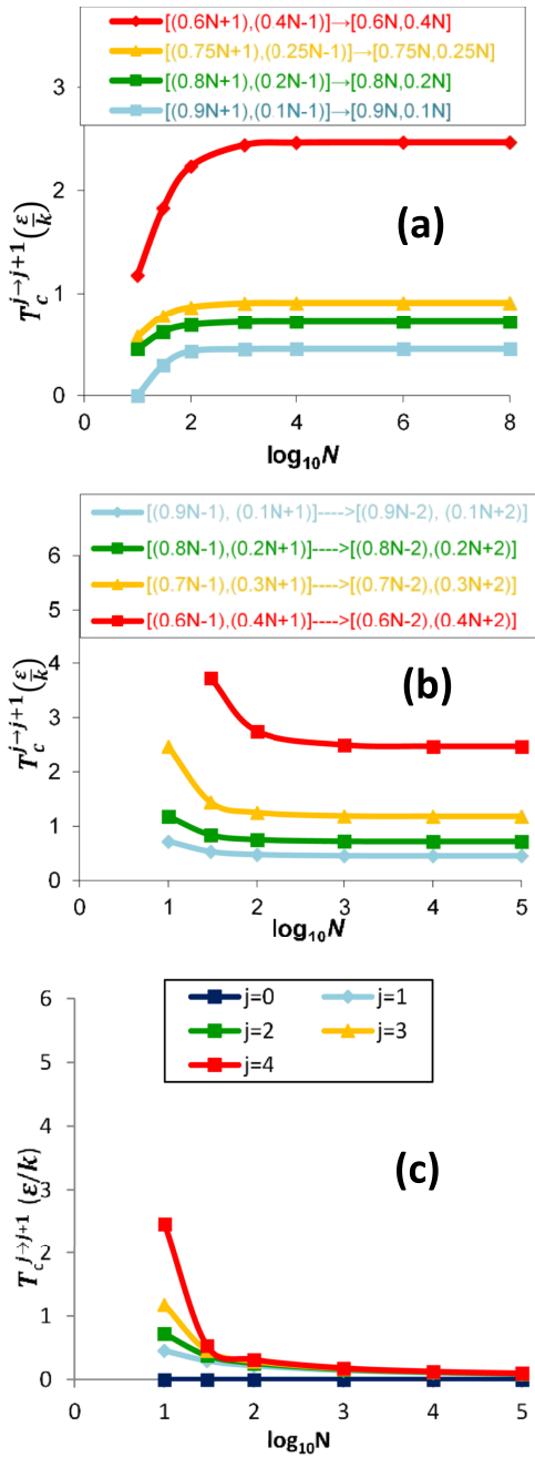
FIG. 4. N -dependence of continuous canonical ESTs for \Delta j = +1 transitions originating from (a) X_j = a - 1/N , increasing- X_j ; (b) X_j = a + 1/N , decreasing- X_j ; and (c) X_j = a/N , decreasing- X_j eigenstates in PSLs.
