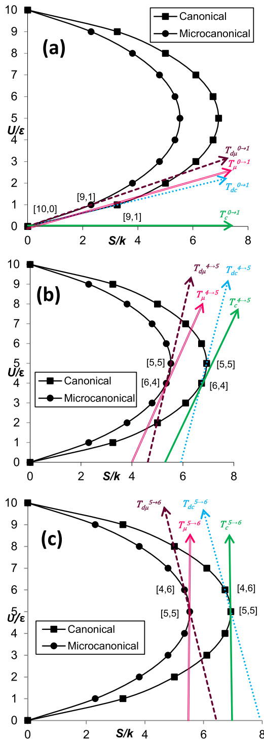
FIG. 2. Continuous microcanonical ( T_{\mu}^{j \rightarrow j+1} ), continuous canonical ( T_c^{j \rightarrow j+1} ), discrete microcanonical ( T_{d\mu}^{j \rightarrow j+1} ), and discrete canonical ( T_{dc}^{j \rightarrow j+1} ) ESTs of the (a) [10, 0] \rightarrow [9, 1], (b) [6, 4] \rightarrow [5, 5], and (c) [5, 5] \rightarrow [4, 6] transitions in an N = 10 PSL. T_{\mu}^{j \rightarrow j+1} and T_c^{j \rightarrow j+1} are equal to the slopes of the tangents to the profiles at the initial points in the transitions; T_{d\mu}^{j \rightarrow j+1} and T_{dc}^{j \rightarrow j+1} are equal to the finite difference slopes between the initial and final points in the transitions.
