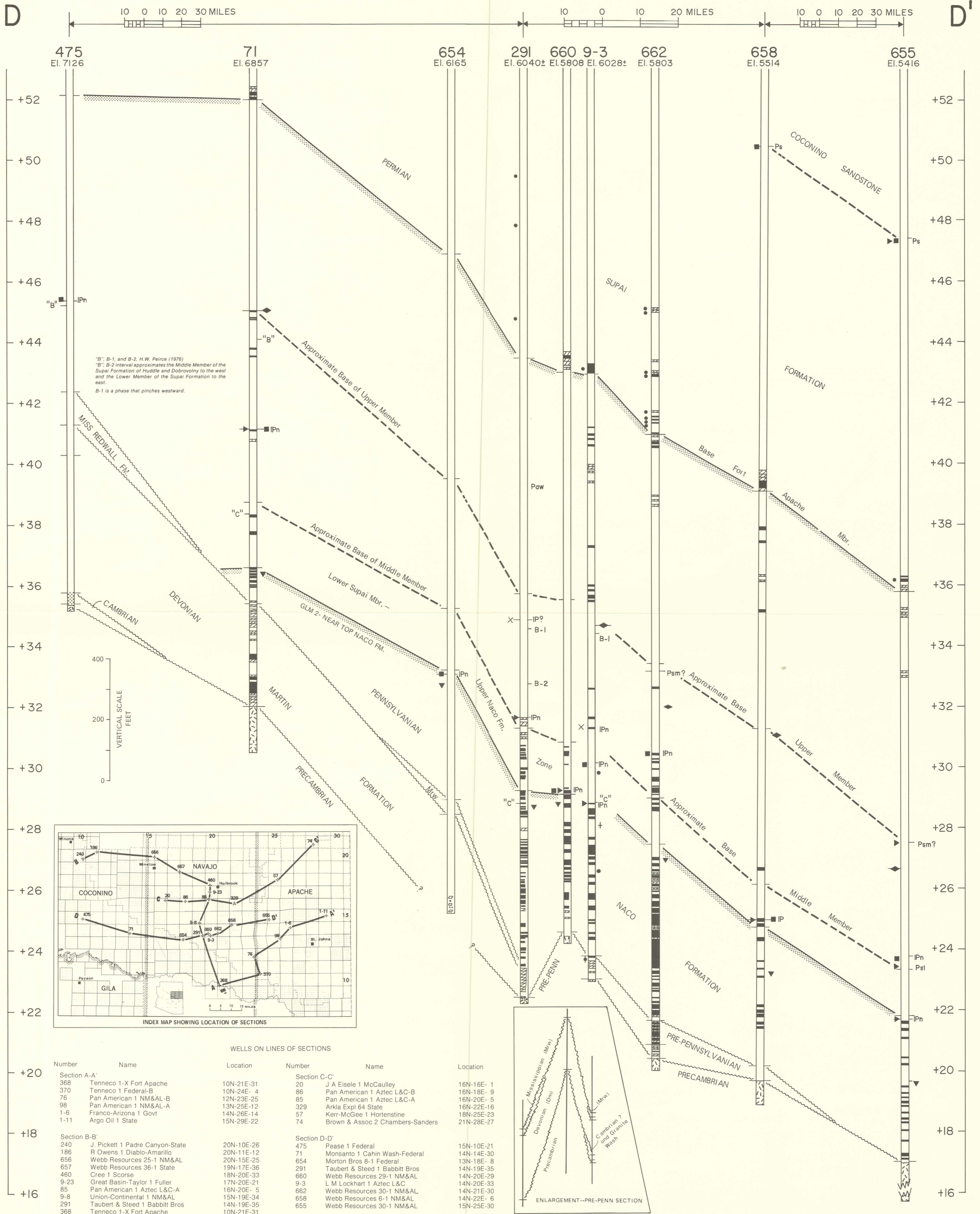
STRUCTURE AND CORRELATION SECTION D-D' EASTERN MOGOLLON SLOPE REGION, ARIZONA
