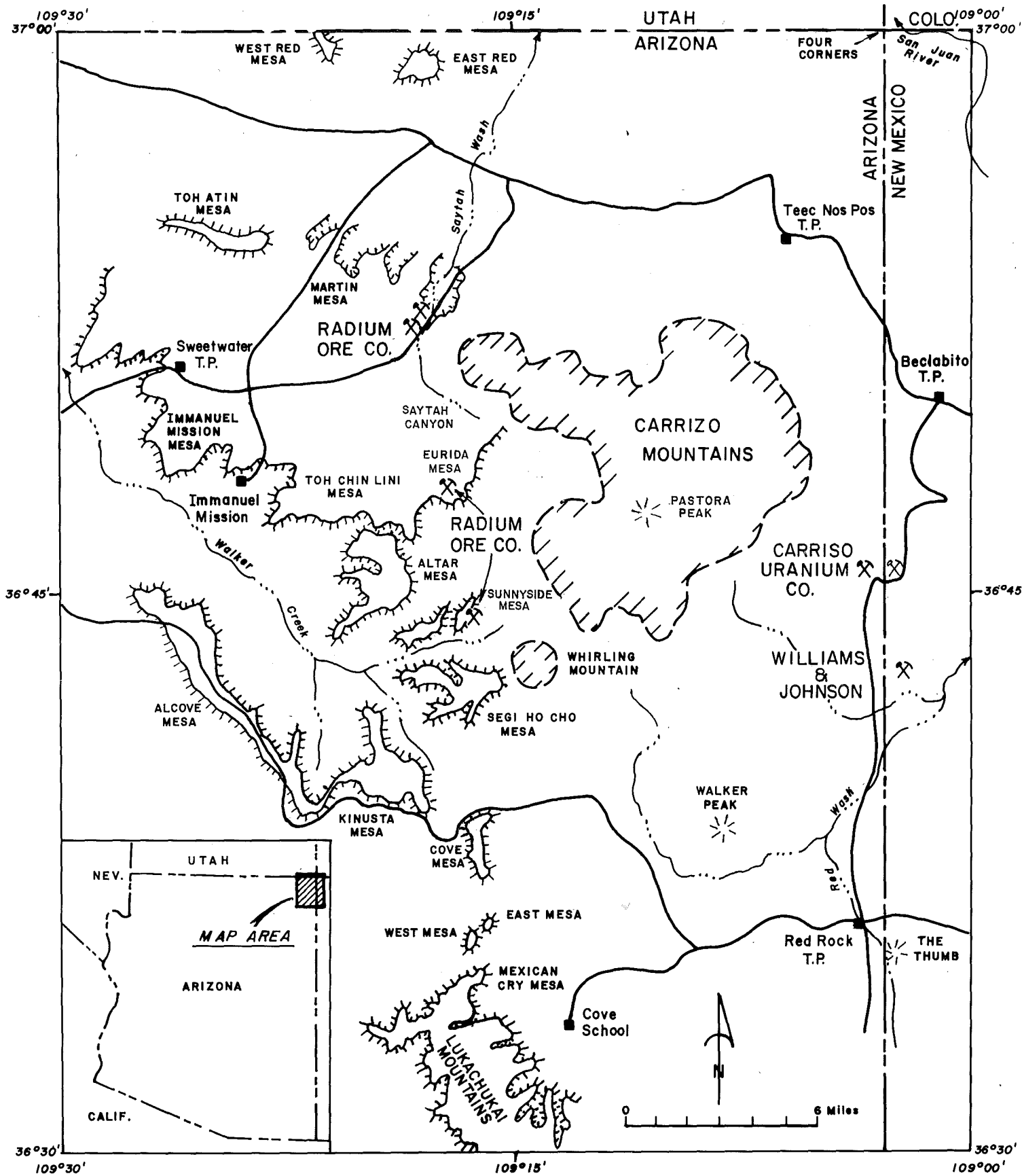
Figure 1. Index map of the Carrizo Mountains showing the location of the carnotite leases issued in the 1920's
