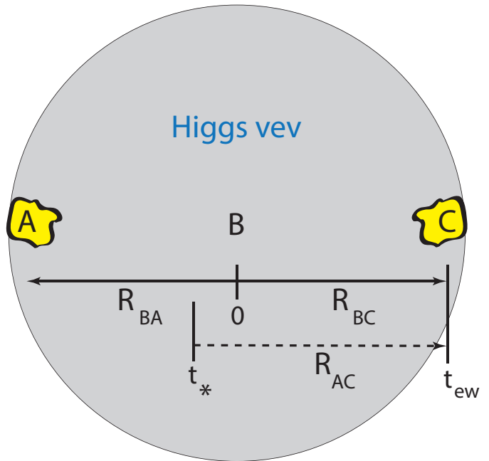
Figure 1. Schematic diagram showing observer B connecting causally with two opposite patches (A and C) in the Higgs vev, a proper distance R_{BA}(t) = R_{BC}(t) away. Patch A emitted a light signal at time t_* that reached C, a proper distance R_{AC}(t_{\text{ew}}) away, at the electroweak phase transition time t_{\text{ew}} .
