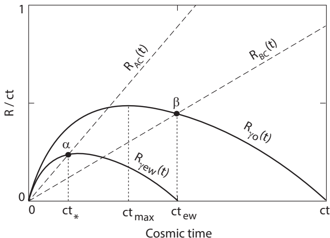
Figure 2. Photon trajectories as seen by an observer in patch C (see fig. 1) for the R_h = ct universe. The curve R_{\gamma_{ew}}(t) represents the null geodesic arriving at C at the electroweak phase transition time t_{ew} from any source emitting light at proper distance R_{src}(t) = R_{\gamma_{ew}}(t) at time t < t_{ew} . The other solid curve R_{\gamma_0}(t) is the null geodesic for light arriving at C at time t > t_{ew} . The dashed lines R_{AC}(t) and R_{BC}(t) show the proper distance from A to C and from B to C, respectively. The other labels and symbols are defined in the text.
