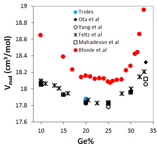
FIG. 5. Molar volume of Ge-Se glasses as a function of composition. Literature data are compared with the value of the ultra-high purity glass produced by Troles et al. 56 While most literature data are in good agreement, the values of Bhosle et al. systematically deviate. This could be attributed to the presence of impurities such as water.
