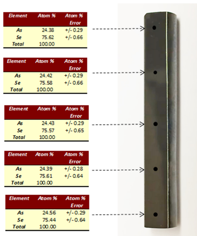
FIG. 2. Quantitative compositional analysis by EDS on five points along an \text{As}_{25}\text{Se}_{75} glass rod produced by melt-rocking. Compositional fluctuations along the rod are well within the experimental error, testifying to the chemical homogeneity of the glass.
