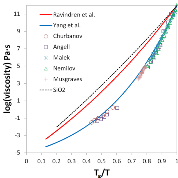
FIG. 6. Fragility plot for \text{As}_2\text{Se}_3 . The red curve is derived from the MYEGA equation using the activation energy of Ravindren et al. , 27 and the blue curve is from that of Yang et al. 64 Experimental viscosity data are from Churbanov, 60 Angell, 62 Malek, 65 Nemilov, 29 and Musgraves. 35 High temperature values were obtained by oscillating cup viscometry.
