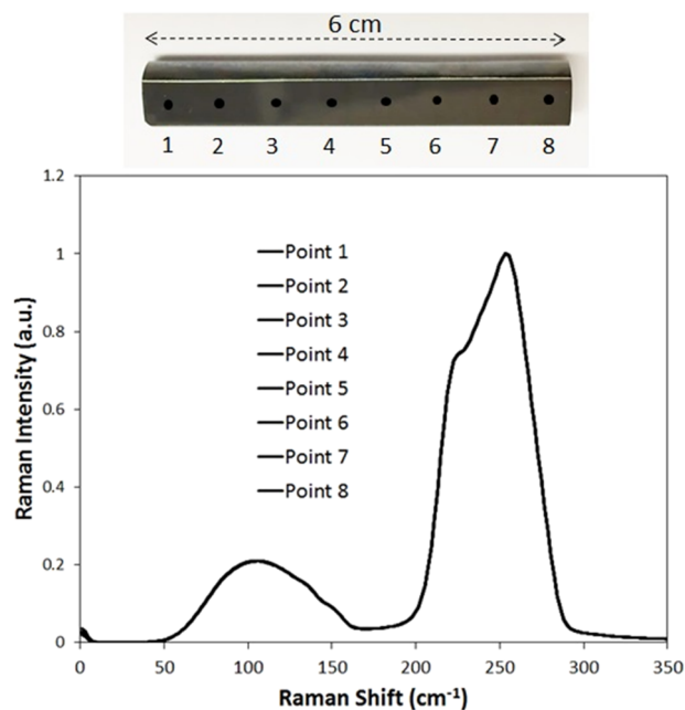
FIG. 1. Intensity-normalized unpolarized Raman spectra collected at eight points along a 6 cm long \text{As}_{25}\text{Se}_{75} glass rod produced by melt-rocking. It is evident that all eight spectra are perfectly superimposable on one another, testifying to the structural and chemical homogeneity of the glass.
