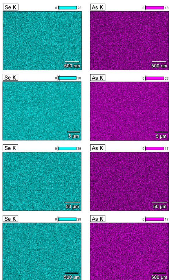
FIG. 3. EDS imaging of an \text{As}_{25}\text{Se}_{75} glass over 4 orders of magnitude in length scale. The Se and As maps demonstrate that the glass is chemically homogeneous at every length scale. The compositional average over each map is also identical at each length scale.
