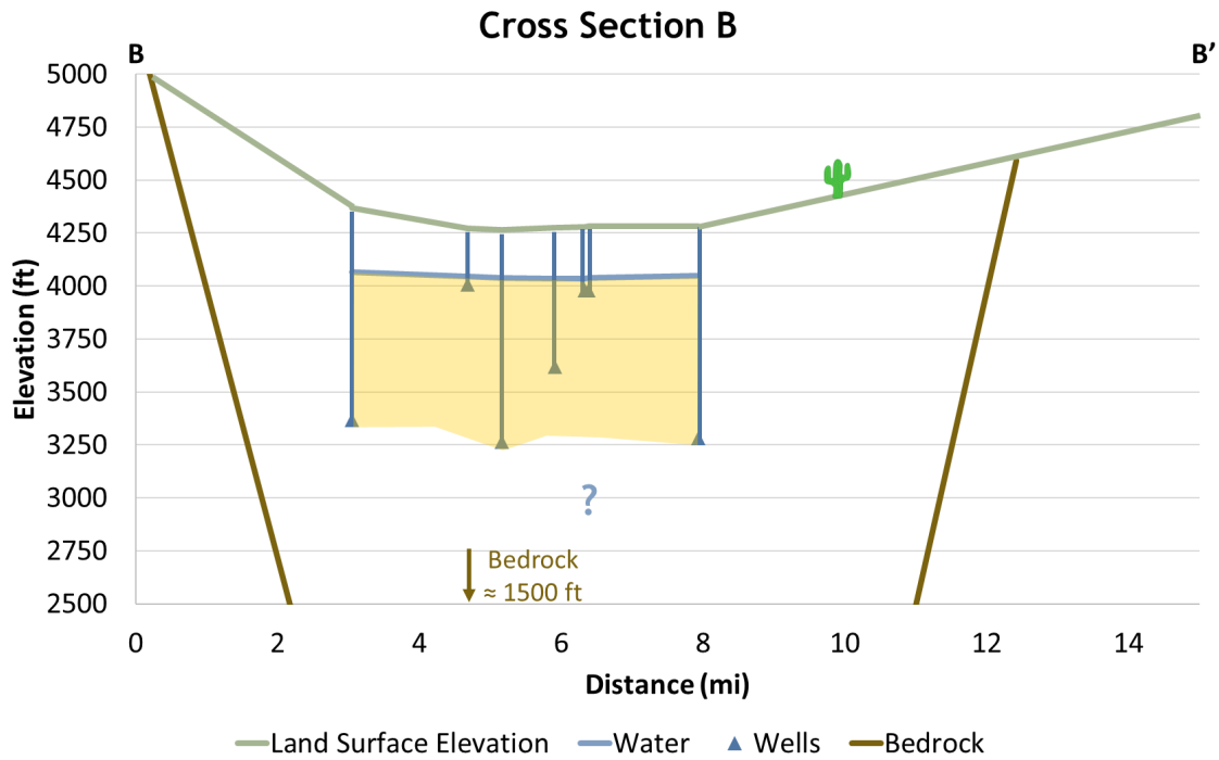
Figure 10. Cross-section B is located north of the Willcox Playa and intersects the northern cone of depression in the Willcox Basin.
