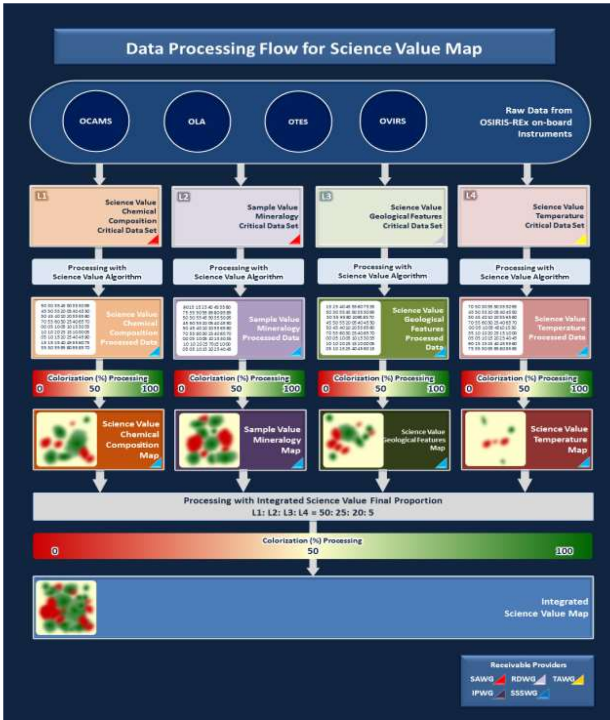
Figure 2: A graphical flow diagram conceptually representing the production of the Integrated Science Value Map.
