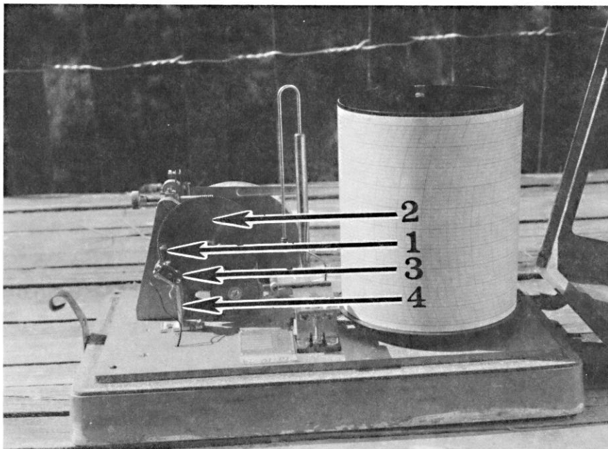
Fig. 1. FW-1 Water Level Recorder with on/off switch. (1) brass lug, (2) gear, (3) micro-switch, (4) alum. H-beam).
