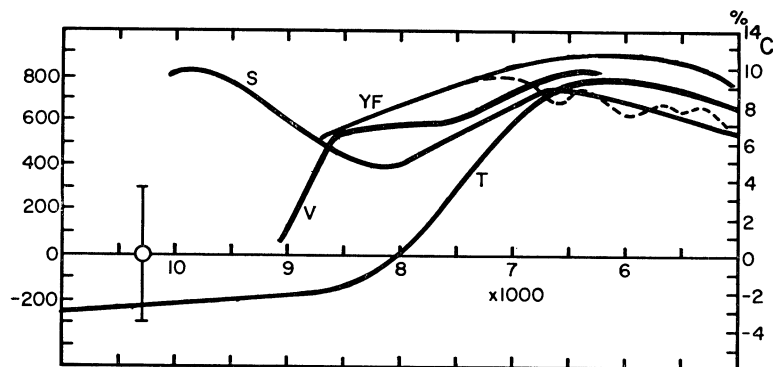
Fig 1. Estimates of the deviation in the ^{14}\text{C} content of the atmosphere between 5000 and 11,000 BP based on varve chronologies. Dashed line is the curve derived from tree rings (Suess, 1970). T: Tauber (1970). Scandinavia. S: Stuiver (1970). Lake of Clouds, Minnesota, USA. V: Vogel (1970). Faulensee, Switzerland. YF: Yang and Fairhall (1971). Saanish Inlet, British Columbia. The end of the Last Glacial, according to the Scandinavian varve chronology, is dated to 10,300 \pm 300 BP, and according to the Northern European pollen diagrams, radiocarbon dated to 10,300 BP (Vogel, 1970) so that, at this point in time, the discrepancy is less than 3 percent.
