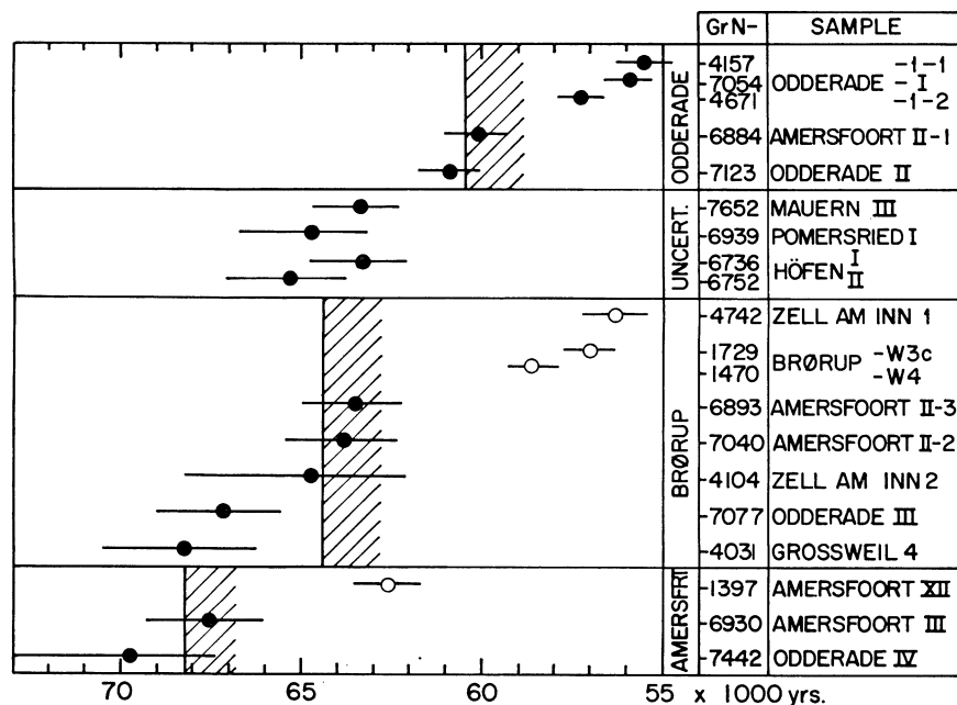
Fig 3. Enriched radiocarbon dates for Early Glacial interstadials in Northern Europe (Grootes, 1977; 1978; Vogel and Zagwijn, 1967). Open circles are dates which must be rejected because they are younger than those for the succeeding stage.
