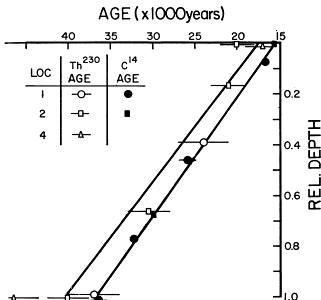
Fig 2. Age of Upper Lisan sediments plotted against relative depth in the sequence. Open signs: ionium dates; closed signs: radiocarbon dates. The best straight lines drawn through the two sets of data deviate by 10 \pm 3 percent from each other.
