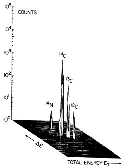
Fig 2. Two-parameter logarithmic plot of a particle spectrum from a graphitic wood sample ( \sim 135\% M) observed with the \Delta E -E heavy ion gas detector. The electrostatic and magnetic analyzing system was set for particles having an energy of 18MeV, charge state 3^+ and mass 14.
