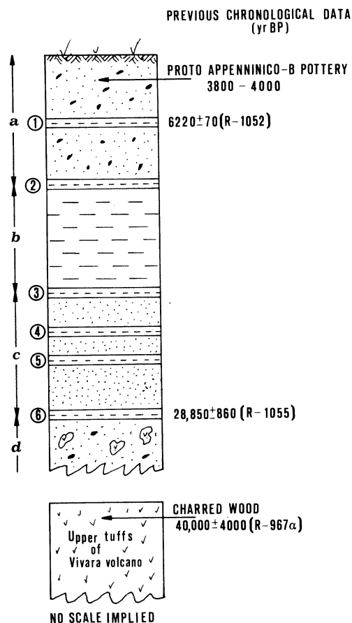
Fig 2. The section exposed at Sancio Cattolico site. The suite of dated PAs (1–6) and the main volcanoclastic terranes are shown. Previous ^{14}\text{C} ages for a charred wood and \text{HA}_{\text{tot}} from PAs # 1 and 6, along with the estimated age for potsherds, are also given. The depicted upper tuffs of Vivara volcano are not exposed in this site. Key: a = Phlegrean tephra; b = Solchiaro formation; c = cinder pyroclasts; d = tephra of Punta della Lingua volcano.
