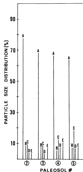
Fig 3. Particle size distribution of the <2 mm fraction for the studied PAs. Key: A = sand (0.05–2 mm); B = coarse silt (20–50 \mu ); C = medium silt (5–20 \mu ); D = fine silt (2–5 \mu ); E = clay (<0.2–2 \mu ).
