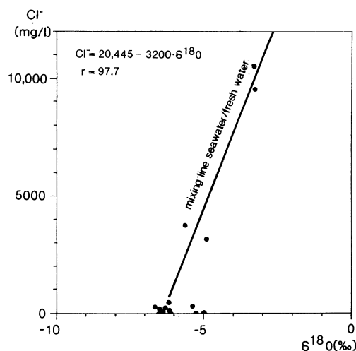
Fig 4. δ 18 O and chloride mixing line for water samples from the Jakarta region
