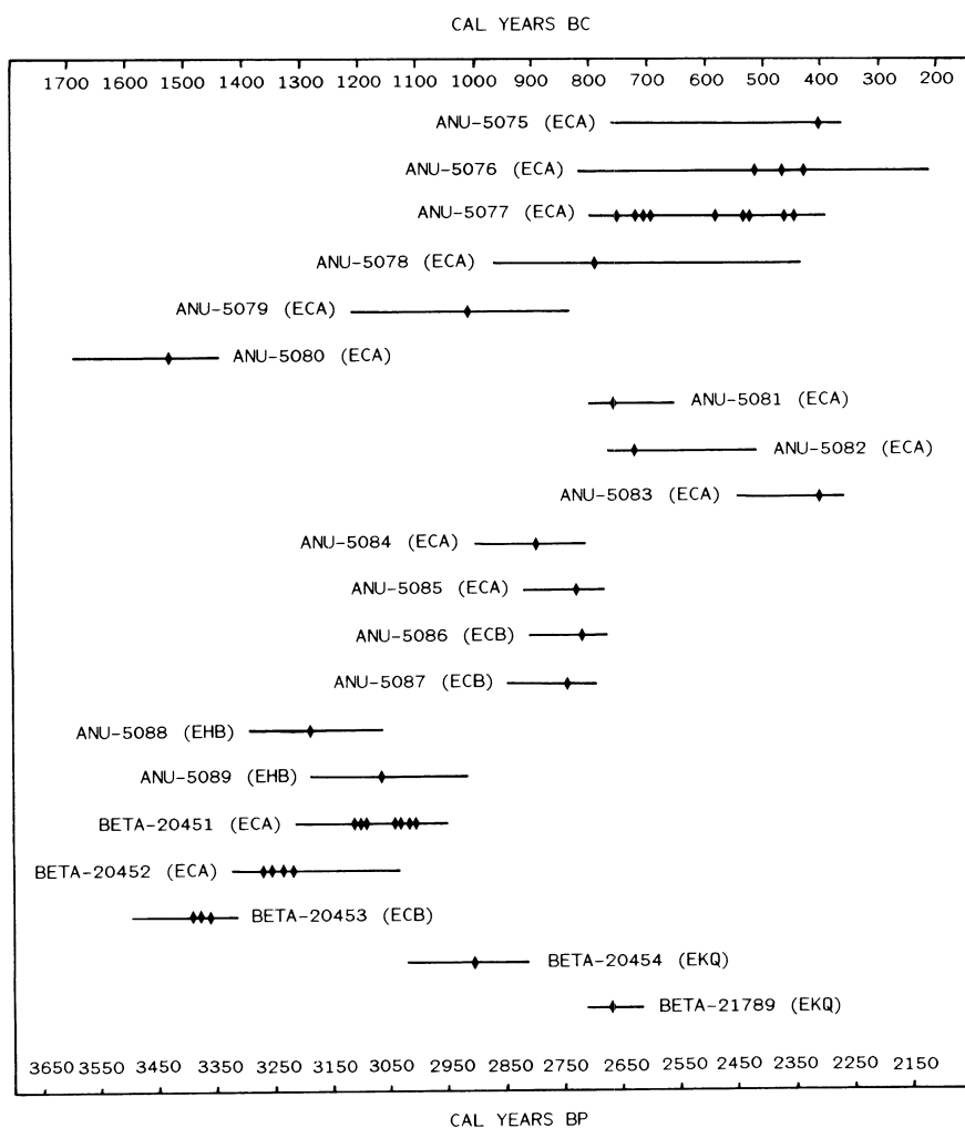
Fig 1. Calibrated age ranges (at 1σ) for 14 C dates from the Mussau Islands Lapita sites. Tick marks indicate intercept points.
