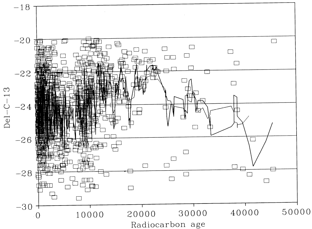
Fig. 4. \delta^{13}C values for all plant categories tabulated from data of the University of Arizona Radiocarbon Laboratory. Lines are 5- and 11-point running means.
