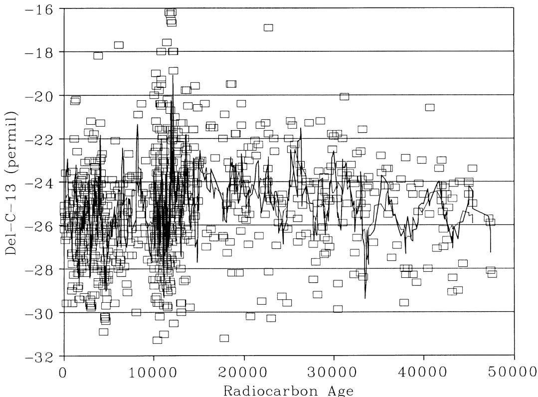
Fig. 2. \delta^{13}\text{C} values ( \square ) for all plant categories tabulated from RADIOCARBON . Five- and 11-point running means are drawn to infer trends.
