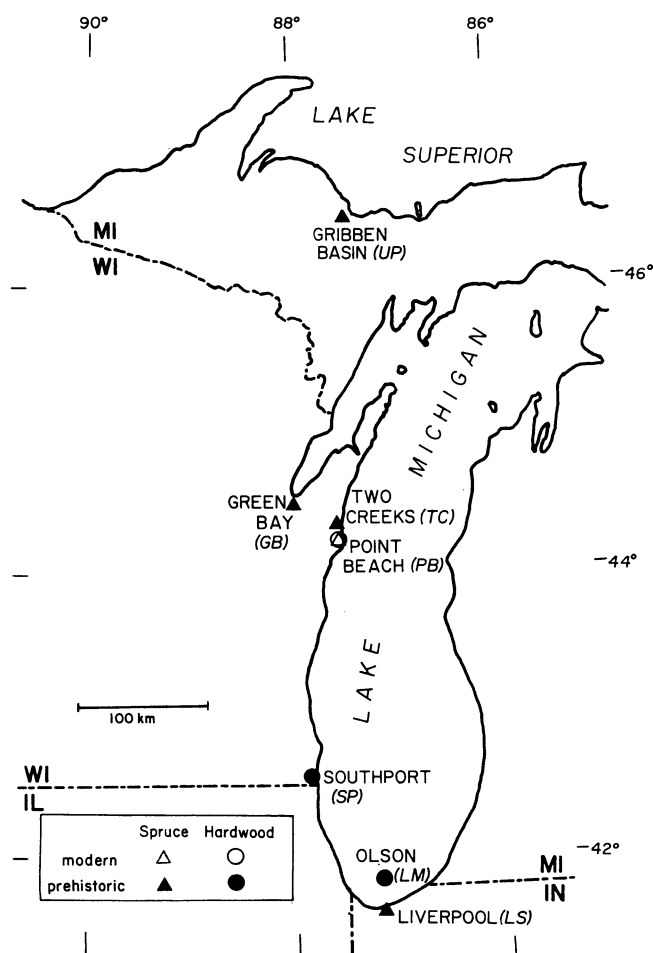
Fig. 1. Site locations where wood was obtained for isotopic analysis in this study. See text for site ages and Table 2 for sample characteristics.
