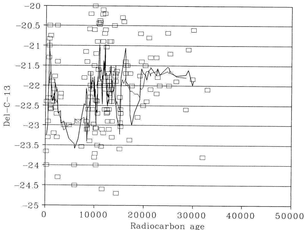
Fig. 5. \delta^{13}\text{C} values for Juniperus data from the Arizona Laboratory. Lines are 5- and 11-point running means.
