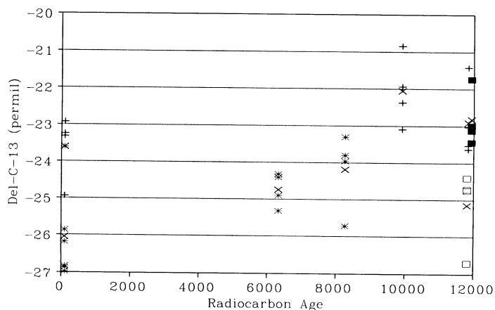
Fig. 6. \delta^{13}\text{C} of wood from six buried forest localities and a modern site. Site locations and abbreviations are shown in Figure 1, and site ages are given in text. ■ = GB spruce; + = TC, UP, PB spruce; * = LM, SP, PB hardwoods; □ = LS spruce; × = averages.
