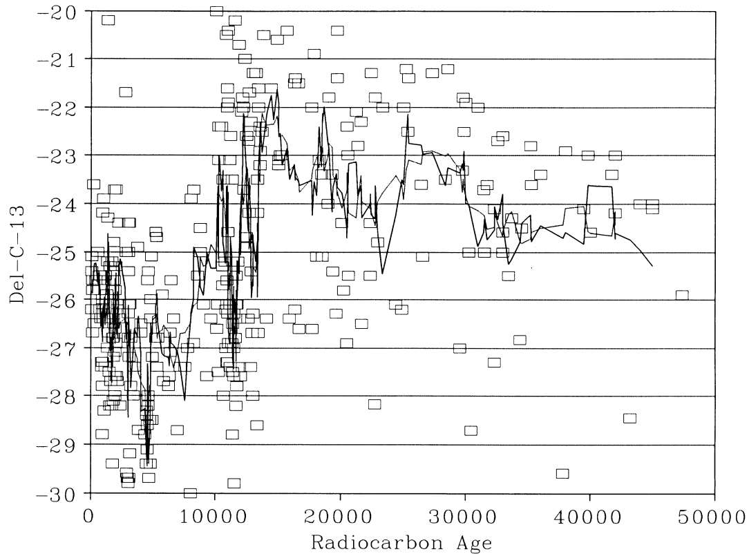
Fig. 3. \delta^{13}\text{C} values for wood samples tabulated from RADIOCARBON . Lines are 5- and 11-point running means.
