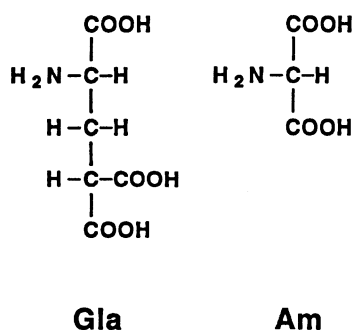
Fig. 1. Structure of gamma-carboxyglutamic acid (Gla) and alpha-carboxyglycine (aminomalonnate) (AM)
