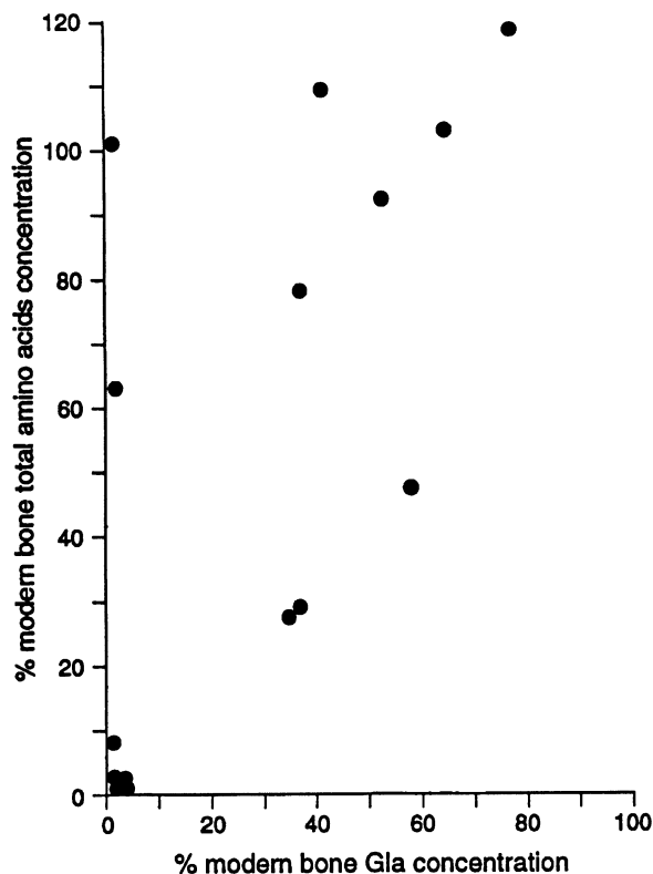
Fig. 2. Relationship of total amino acids and Gla concentrations in a series of fossil bones expressed as a percentage of total amino acids and Gla in a modern bone standard.
