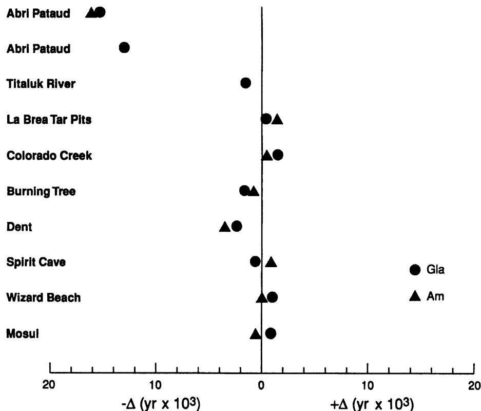
Fig. 3. Age offset (in yr × 10 3 ) between Gla and Am and total amino acid fractions
