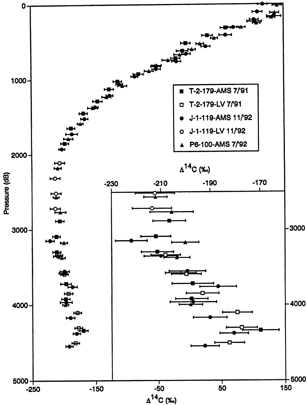
Fig. 2. Comparison of AMS and LV results for three stations in the south-central Pacific Ocean. The TUNES-2 station 179 data and the Juno-1 station 119 data were collected at the same location (33°S, 135°W), but 14 months apart (7/1991 and 11/1992, respectively). The P6 station 100 data (7/1992) were collected ca. 250 nautical miles (463 km) away (32.5°S, 130°W). The insert shows data from the bottom 2500 dB on an expanded scale. Both LV and AMS techniques were employed on the TUNES and Juno cruises while only AMS was used on P6. No systematic difference in techniques is evident for these data.
