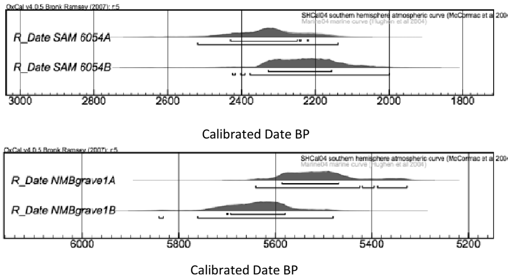
Figure 4 Observed % Marine values used to calibrate 14 C dates for both Modder River (SAM 6054) and Matjes River (Grave 1) samples.
