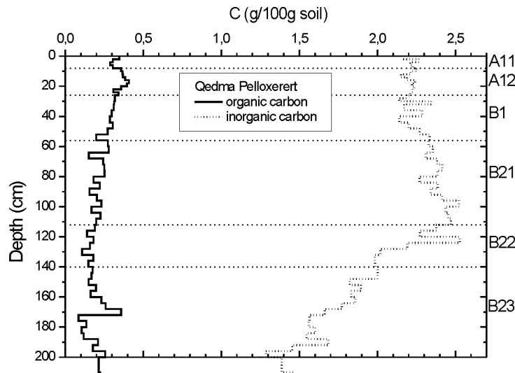
Figure 1 Organic and inorganic carbon, Qedma profile
