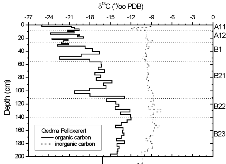
Figure 3 \delta^{13}\text{C} of organic and inorganic carbon, Qedma profile
