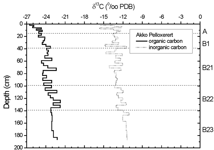
Figure 6 \delta^{13}\text{C} of organic and inorganic carbon, Akko profile
