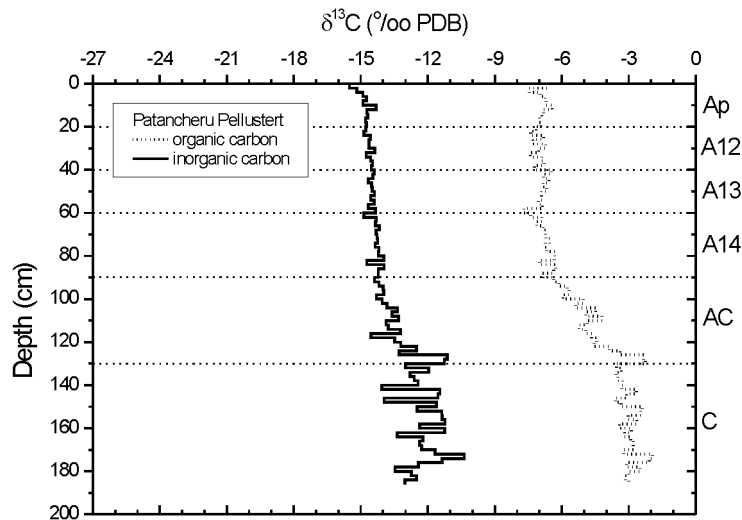
Figure 9 \delta^{13}\text{C} of organic and inorganic carbon, Patancheru profile
