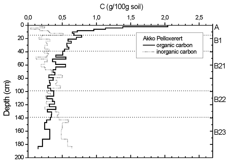
Figure 4 Organic and inorganic carbon, Akko profile
