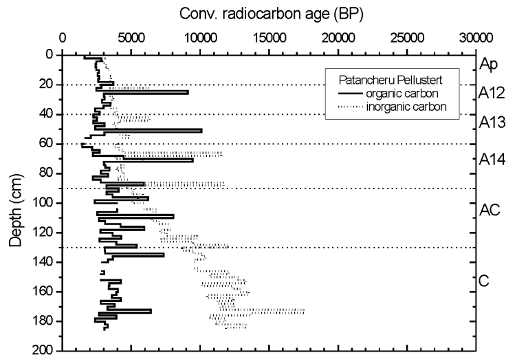
Figure 8 ^{14}\text{C} age of organic and inorganic carbon, Patancheru profile
