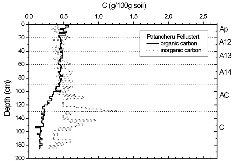
Figure 7 Organic and inorganic carbon, Patancheru profile
