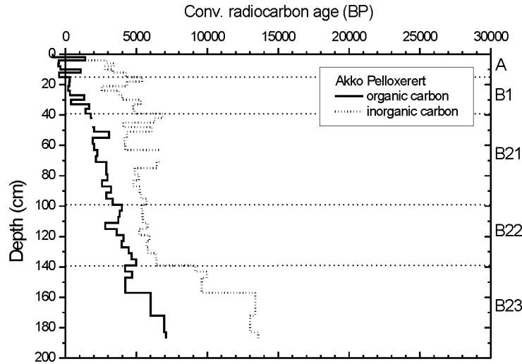
Figure 5 ^{14}\text{C} age of organic and inorganic carbon, Akko profile
