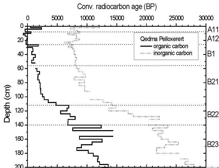
Figure 2 ^{14}\text{C} age of organic and inorganic carbon, Qedma profile
