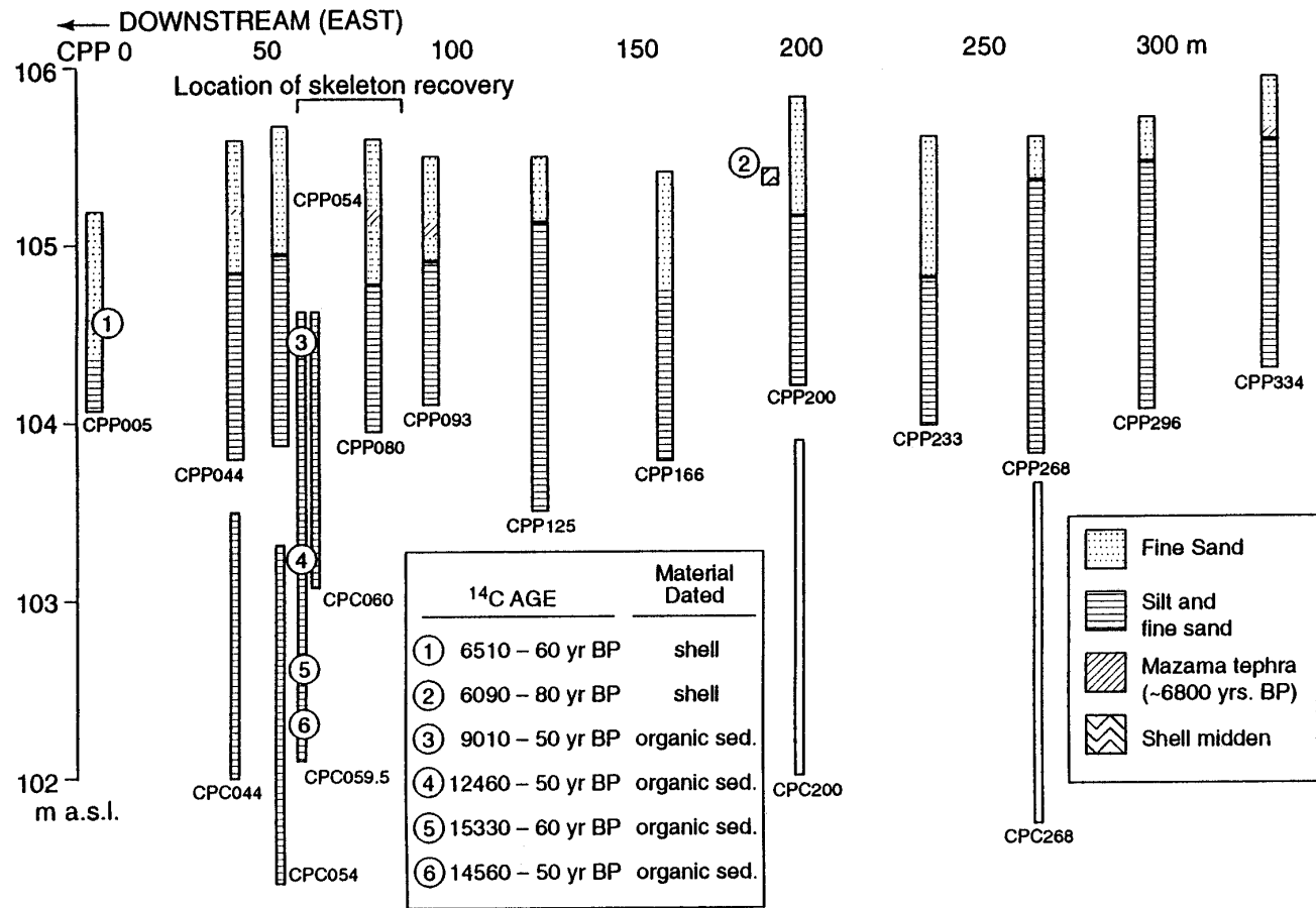
Figure 1 Fence diagram of stratigraphy at the Columbia Park site, Kennewick, Washington, in relationship to 14 C determinations of freshwater shell and humates and the occurrence of Mt Masama tephra. Radiocarbon determinations (from Wakeley et al. 1998): (1) 6510 ± 60 BP: Beta-11383 [shell]; (2) 6090 ± 80: Beta-113977 [shell], (3) 9010 ± 50 BP: WW-1626 [sediment organics], (4) 12,460 ± 50 BP: WW-1738 [sediment organics]. Adapted from Huckleberry and Stein (1999:Figure 1).
