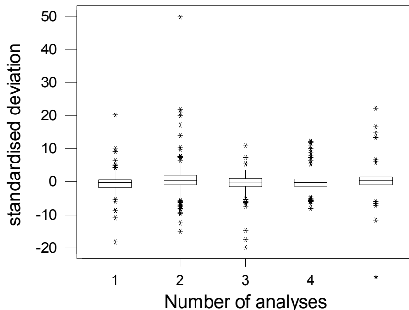
Figure 7.18 Distribution of standardized deviations by number of laboratory analyses
