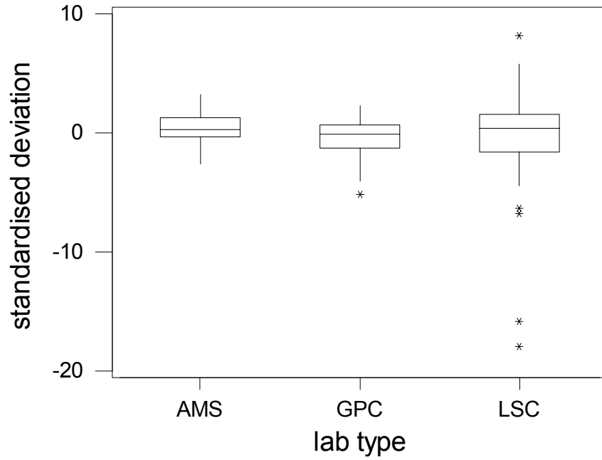
Figure 7.9 Distribution of standardized deviation for Sample D
