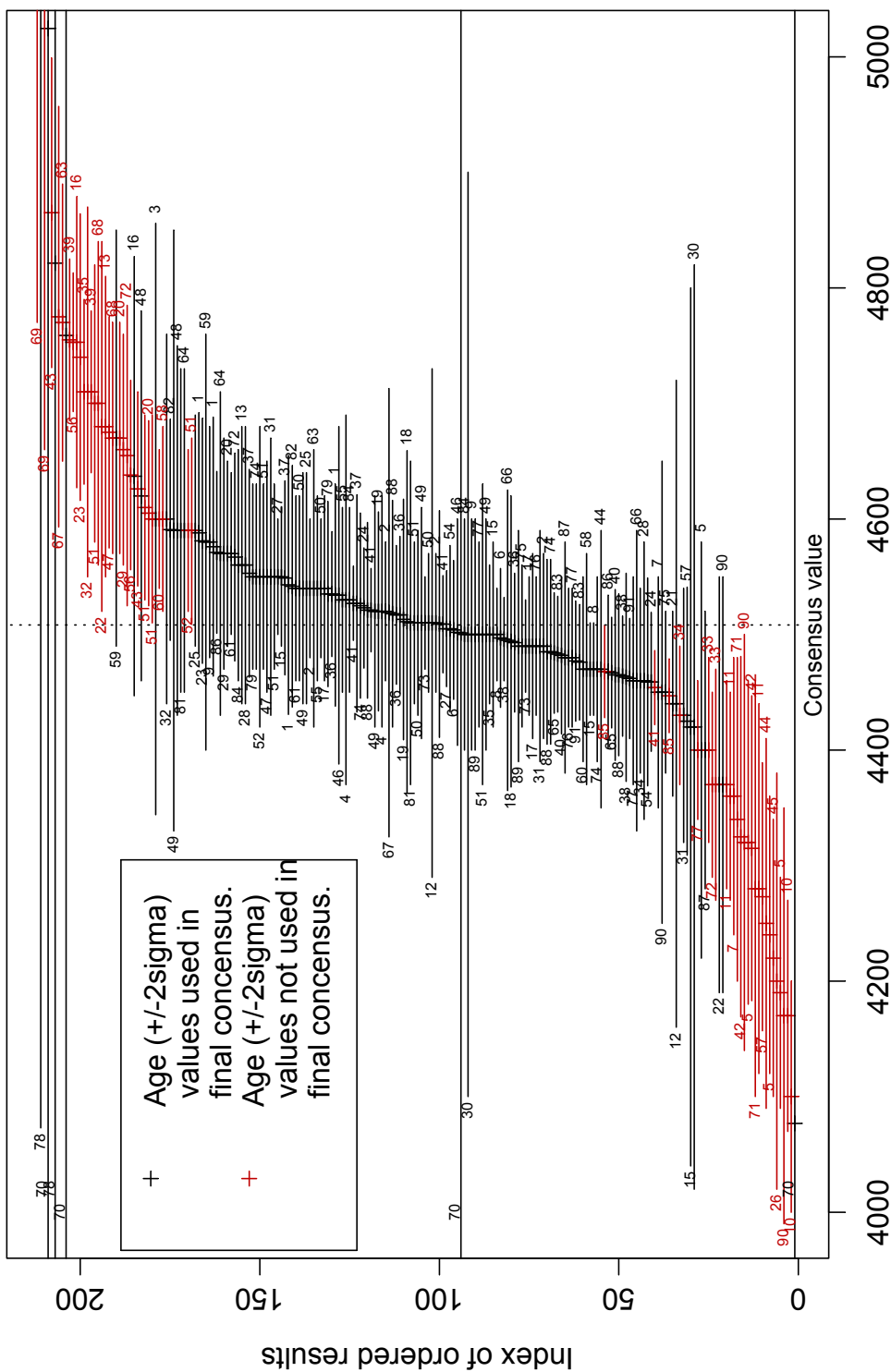
Figure 7.3 Distribution plot of Belfast dendro-dated wood, D & F, age with consensus value for all laboratories
