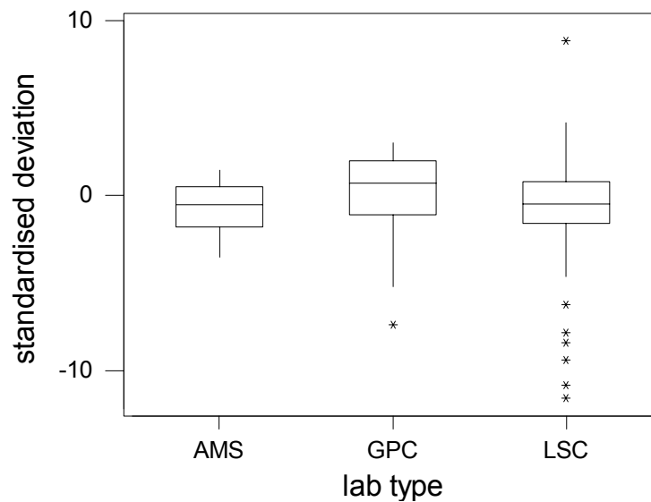
Figure 7.12 Distribution of standardized deviations for Sample G
