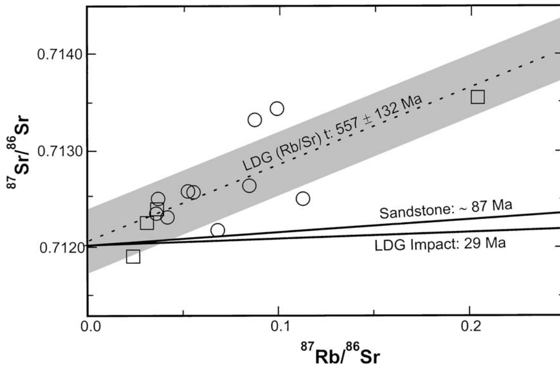
FIG. 4. Rb-Sr isotopic evolution diagram for 14 LDG samples. A linear regression through all sample points yields an age of 557 \pm 132 Ma with an initial ^{87}\text{Sr}/^{86}\text{Sr} ratio of 0.71209 \pm 0.00015 . Shaded area corresponds to the deviation ( \pm 1\sigma ) of the ^{87}\text{Sr}/^{86}\text{Sr} values. Reproducibility error bars for the samples are smaller than the symbols. Reference lines corresponding to 29 Ma (impact event) and to \sim 87 Ma (stratigraphic age of the Saad Sandstone Formation) are also plotted. For symbols see Fig. 2.
