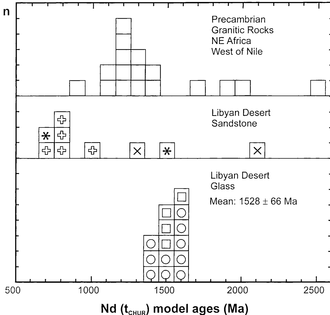
FIG. 8. Nd(t_{CHUR}) model age histogram for 14 LDG samples (bottom), Libyan Desert sandstones from the LDG strewn field and BP and Oasis craters (middle) and Precambrian granitic rocks (top). For symbols see Fig. 2, data sources for granitic rocks see Fig. 6.
