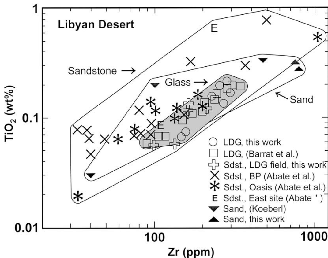
FIG. 2. Zr (ppm) vs. TiO 2 (wt%) diagram for LDG, sandstone and surface sand samples from the Libyan Desert. Data are from this work (Table 1) and from literature: Barrat et al. (1997, LDG samples); Abate et al. (1999, BP and Oasis craters and east of these craters (E)); Koeberl (1997, surface sand). LDG samples define a compact (shaded) field within the surface sand and sandstone sample fields, including 12 sandstone samples. Twenty other sandstone samples and all surface sand samples plot outside the LDG field.
