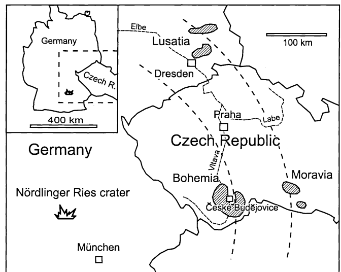
FIG. 1. Schematic map of moldavite occurrences (hatched areas) in Bohemia, Moravia and Lusatia, formed by the Nördlinger Ries impact event (not included are minor occurrences in Lower Austria, the Cheb area and elsewhere; cf., Koeberl et al. , 1988; Lange, 1996; Bouška, 1998).
