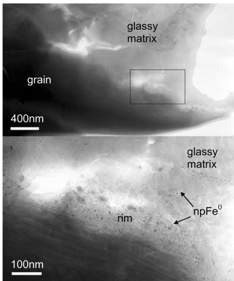
Fig. 6. a) A TEM bright field image of an npFe 0 -bearing rim that is degrading into the surrounding glass; b) a close-up image of the boxed region.
