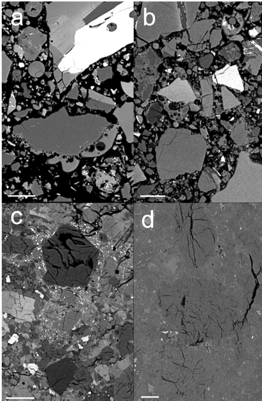
Fig. 1. SEM BSE images of lunar regolith breccia samples: a) 79035; b) 10068; c) 15505; and d) QUE 93069 (as a highland breccia, this sample is largely plagioclase and therefore displays little contrast in backscatter). Note the decreasing porosity from (a) to (d). All scale bars are 20 \mu\text{m} .
