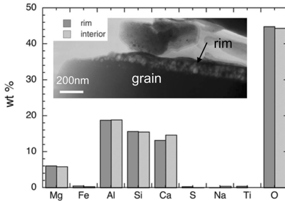
Fig. 8. This vesicular rim from 79035 is compositionally identical to the grain interior. The data are from EDX spectra.
