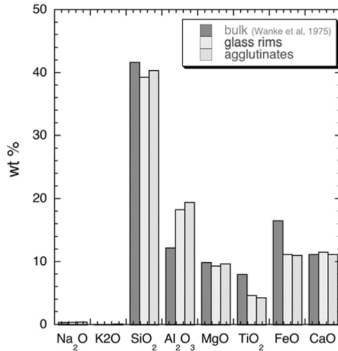
Fig. 11. Glass rims in 79035 are similar in composition to 79035 agglutinitic glass from the same thin section. Bulk data from Wänke et al. (1975).
