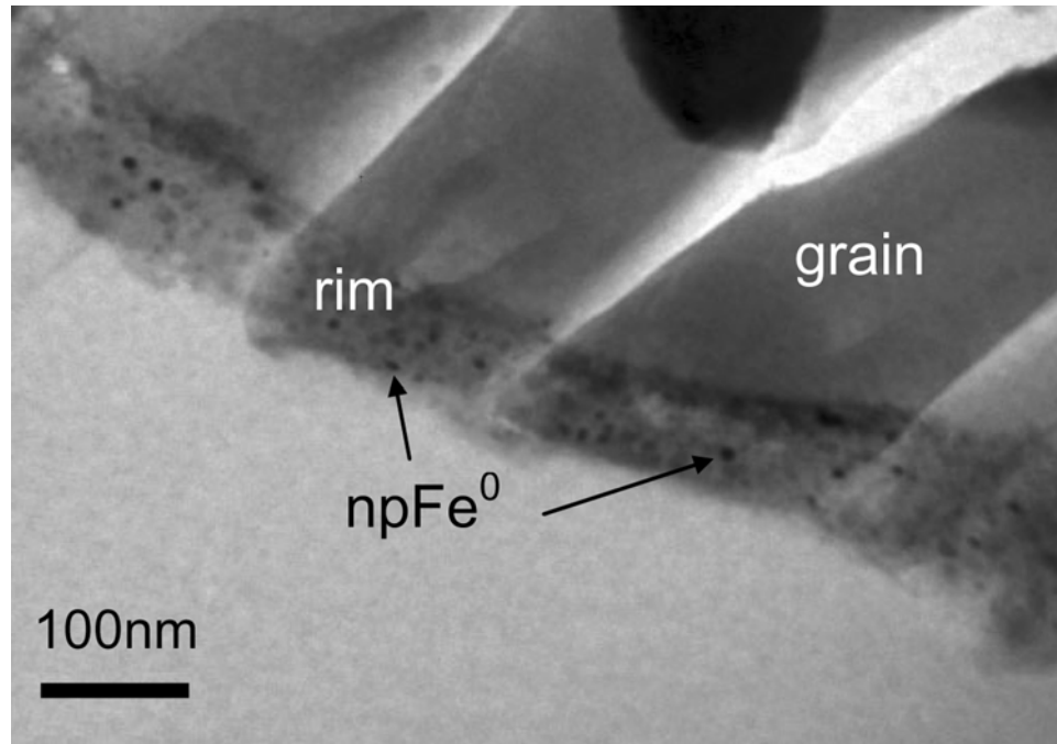
Fig. 4. A TEM bright field image of an npFe 0 -bearing rim from the moderately coherent lunar regolith breccia 10068. The sample was prepared from a microtomed section.
