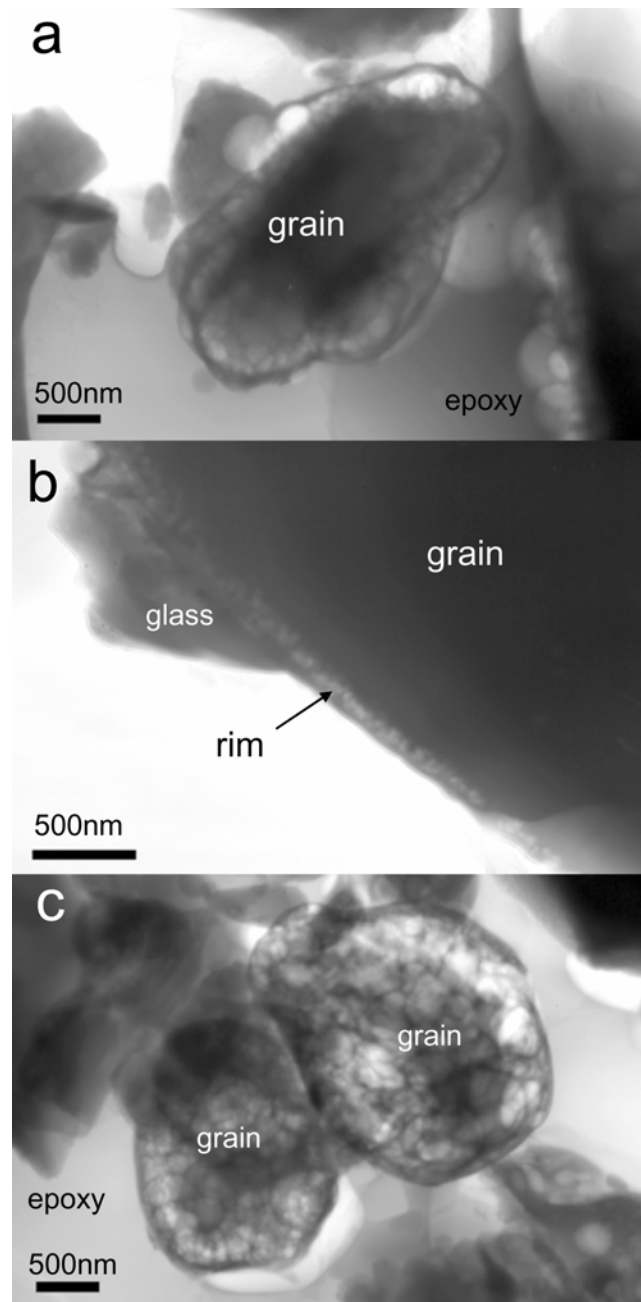
Fig. 7. Examples of vesicular rims: a) a continuous vesicular rim from 79035; b) a partially vesicular grain from 79035; c) two completely vesicular grains from 79035.
