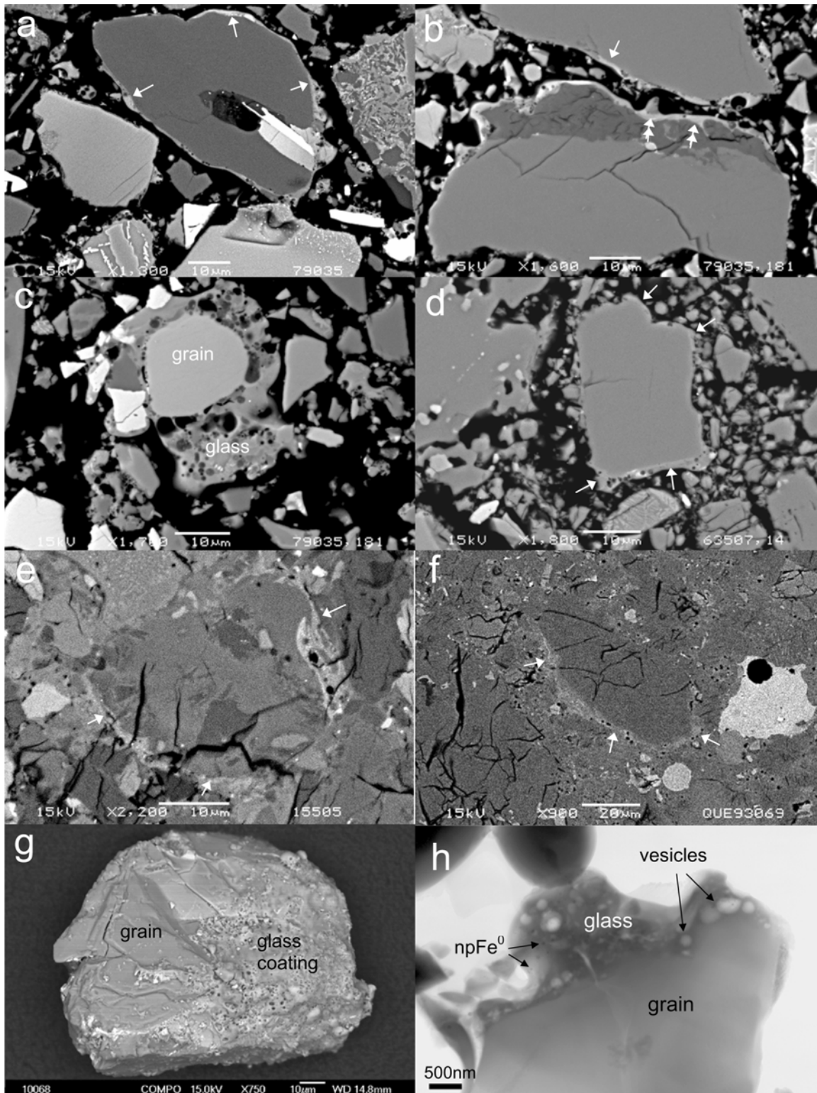
Fig. 10. Examples of glass rims: a) multi-lithic grain from 79035 completely incased in a glass rim; b) two grains from 79035 with glass rims (note especially the obvious flow textures highlighted by double arrows); c) a pyx grain from 79035 that is surrounded by vesicular glass with incorporated lithic components; d) a plagioclase grain from highland soil 63507; e) a plagioclase grain from 15505 with a nearly complete rim; f) a glass rim from QUE 93069; g) a plagioclase grain from the disaggregated 10068 (this grain is approximately two-thirds coated with glass); h) a TEM bright field image of a glass rim from 79035.
