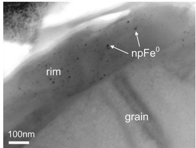
Fig. 3. A TEM bright field image of a \text{npFe}^0 -bearing rim from friable lunar regolith breccia 79035.
