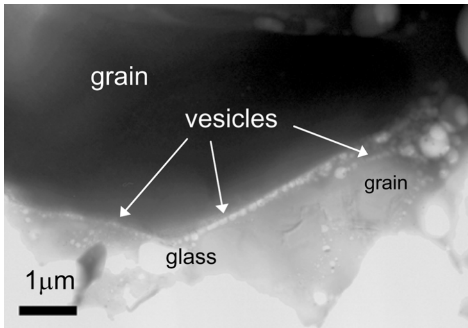
Fig. 9. A TEM bright field image of an agglutinate with imbedded grains from lunar regolith breccia 79035. A line of vesicles is often found at the interface between glass and crystal in these breccias.
