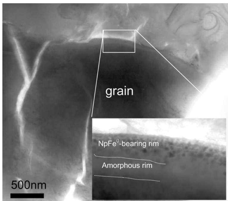
Fig. 5. A TEM bright field image of a multiple rim (amorphous + npFe 0 -bearing) from the very coherent lunar regolith breccia 15505.
