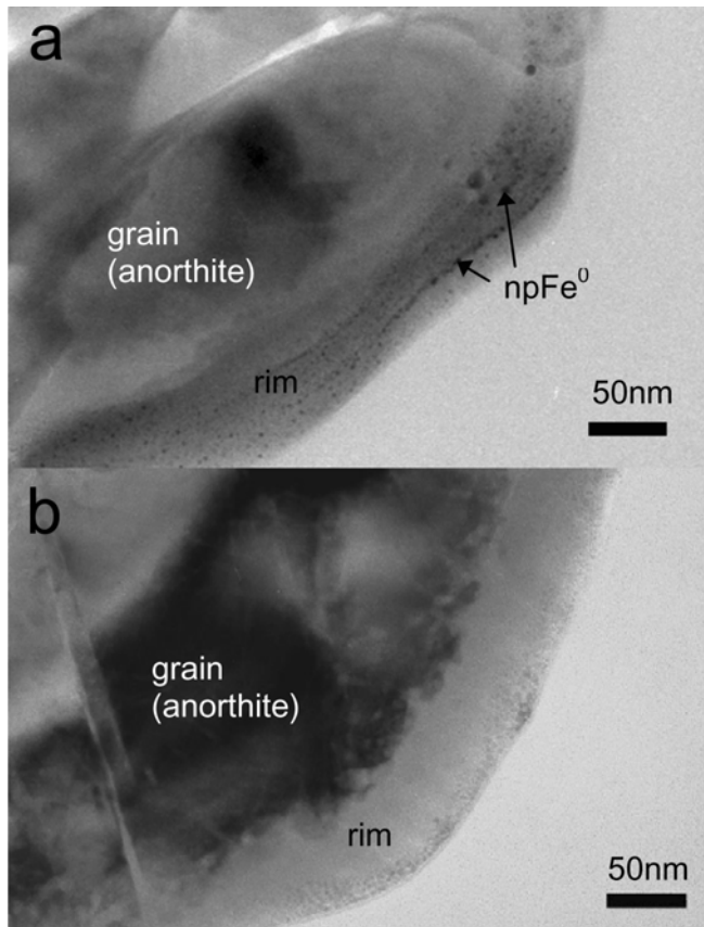
Fig. 2. a) A TEM image of a grain of lunar soil 10084 with a \text{npFe}^0 -bearing-rim. b) A TEM image of a grain of lunar soil 78221 with an amorphous rim.
