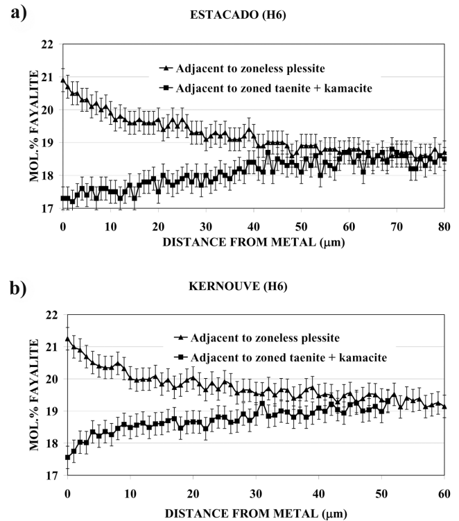
Fig. 5. (a) and (b) report olivine composition as a function of distance from Fe-Ni metal. Analyses represented by squares were collected while traversing olivine toward zoned taenite + kamacite particles; analyses represented by triangles were collected while traversing olivine toward zoneless plessite particles. Olivine-metal interfaces are positioned at the left (distance = 0 \mu\text{m} ).
