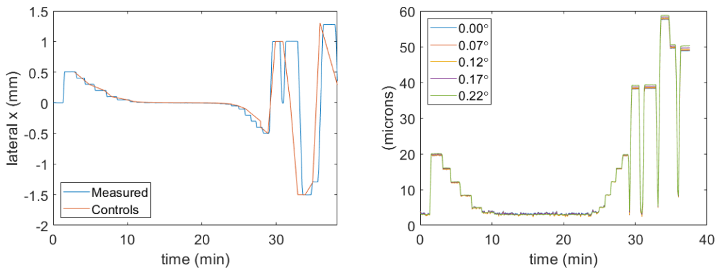
Figure 8 The effect of lateral x decenter (left) on the image RMS spot size (right). Using TMS pose data the spot size is determined across several fields and is found to correlate well to the induced lateral motion.
