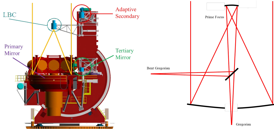
Figure 1 (left) Prime focus is engaged for use with the Large Binocular Camera (LBC). The telescope is pictured at zenith. Elevation changes occur along the c-ring structure. (right) Each mirror has three focus modes: prime focus, Gregorian, and bent Gregorian. Prime focus has a single focal station operating at F/1.142. The Gregorian and bent Gregorian operate at F/15 [2].
