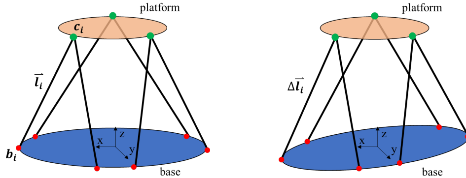
Figure 5 The Stewart-Gough platform in its initial position consists of a platform held parallel to a base supported by legs of length l (left). Changes in leg length \Delta l are made to move the platform to a desired position and orientation relative to the stationary base (right).
