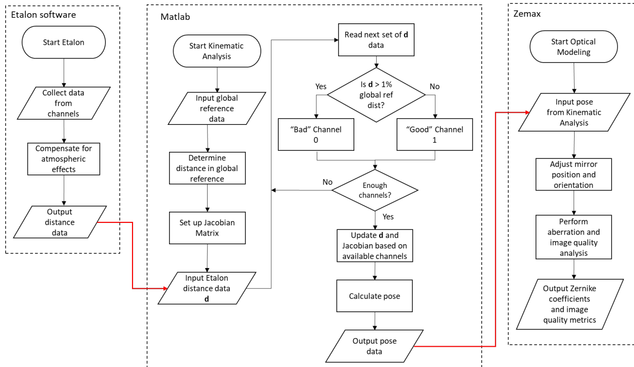
Figure 4 Data pipeline from the Etalon Absolute Multiline Technology to kinematic analysis performed in MATLAB to image quality and aberration analysis in Zemax OpticStudio. Currently the process is modular, with each program working independently. The red arrows indicate a transfer of data from one program to the next, which is performed manually.
