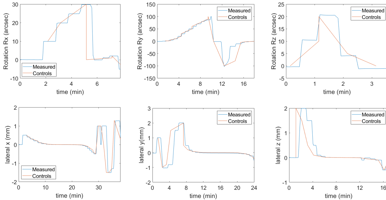
Figure 6 TMS data for Rx, Ry, and Rz rotational (top) and x, y, and z lateral motion (bottom). In all plots the red line represents the induced motion of the primary mirror and the blue line corresponds to the measured change in position and orientation. For all controlled steps in motion TMS determined the corresponding pose, although there is some delay due to different sampling times between TCS and TMS.
