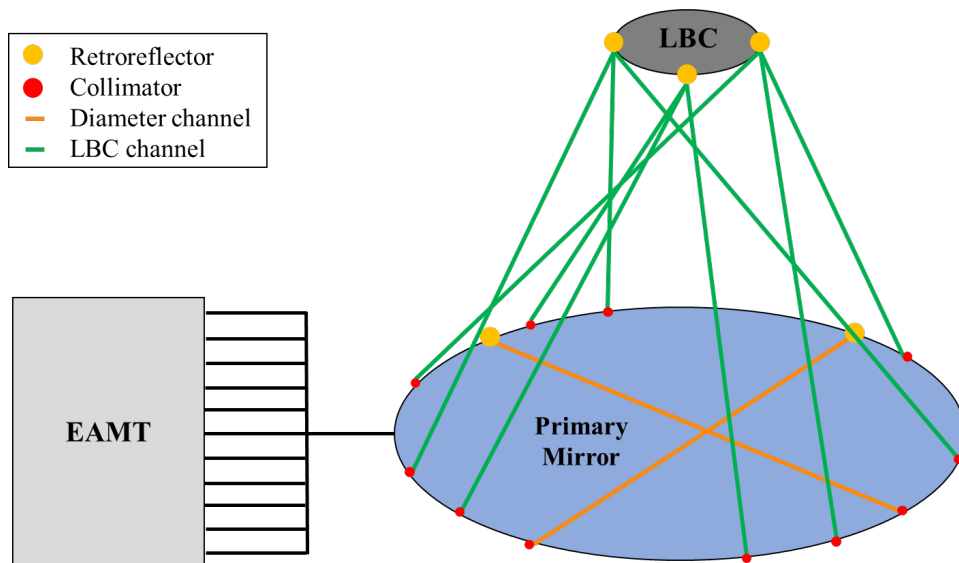
Figure 3 Collimator and retroreflector scheme on TMS. Fiber channels are routed from the EAMT to the collimators around the primary mirror. The collimators are aligned to three retroreflectors on LBC to create the laser truss. Two retroreflectors on the primary mirror are used to monitor the diameter of the mirror.
