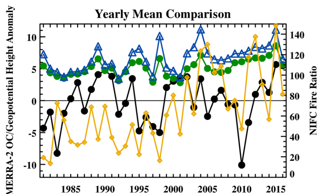
Figure 6. The 1981–2016 MERRA-2 domain mean yearly surface organic carbon mass concentration (green circle line), warm season domain mean OC concentration (blue triangle line), and 850-hPa isobaric height domain mean anomaly (black circle line). The National Interagency Fire Center (NIFC) fire number ratio (gold diamond line) is plotted on the secondary y axis. Note that the NIFC product does not include fire data from Canada and Mexico which likely contributes to the lower correlation with the MERRA-2 products. However, positive isobaric anomalies (increased synoptic ridging) do seem to facilitate conditions of carbonaceous aerosol abundance more often than negative anomalies, especially since 2010.
