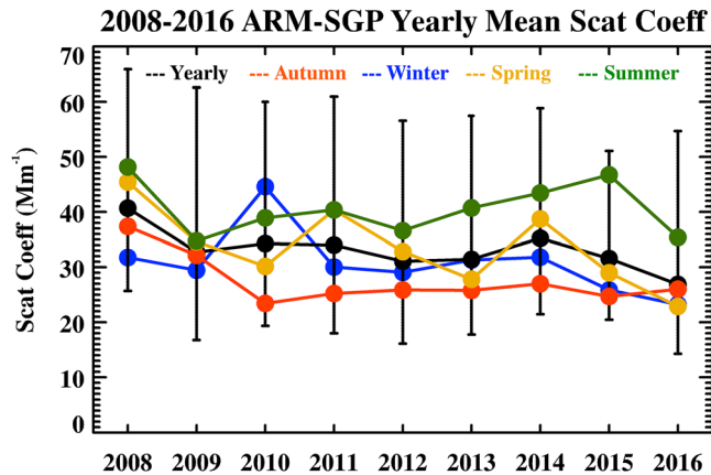
Figure 4. Yearly (black) and seasonal (winter-blue, spring-gold, summer-green, and autumn-orange) mean aerosol observation system (AOS) scattering coefficient trend. Note the decreasing trend of mean yearly and seasonal aerosol loading except for the summer season. In addition, the summer maxima in biomass burning smoke aerosols (North American wildfire activity) are also captured by the AOS. The black bars denote the IQR for the year.
