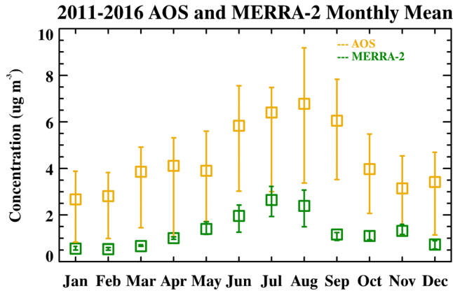
Figure 2. Monthly mean (box) carbonaceous concentrations from the (a) aerosol observation system (AOS) (2011–2016) and (b) MERRA-2 (2011–2016) platforms. Note that the summer maximum in carbonaceous aerosols is captured by both platforms due to wildfire activity within North America. The bars denote the IQR as in Figure 1.
