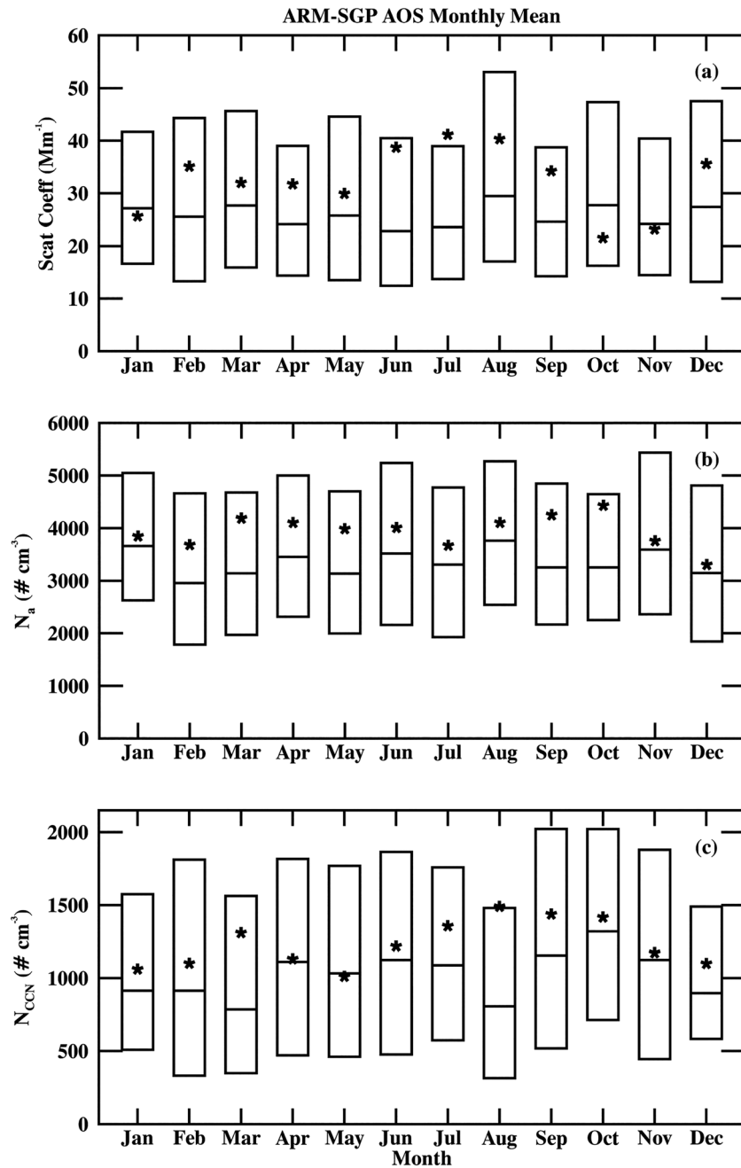
Figure 1. The 2008–2016 monthly mean (asterisk) and median aerosol observation system (AOS) (a) scattering coefficient, (b) aerosol number concentration ( N_a ), and (c) cloud condensation nuclei number concentration ( N_{\text{CCN}} ). The interquartile range (IQR) is added to show the spread of the AOS measurements. Note the seasonality of the data set which is more positively skewed during the summer and autumn (JJASO) months with a second maximum from late winter through the spring (FMAM).
