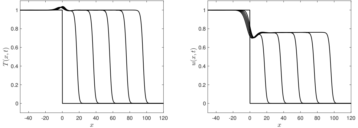
Figure 2: Temporal evolution of system (1.2) at \nu = \rho = 1 with Heaviside initial conditions. Profile snapshots are provided at t = 0, 10, 20, 30, 40, 50 with the waves propagating to the right with asymptotic speed 2. With these values we have u_0 \approx 0.76393 , represented at the elongating middle plateau of the u(x, t) component. It is important to note here that the steady state selected at the back of the emerging wave in u(x, t) corresponds to u_0 = c + \rho - \sqrt{c^2 + \rho^2} instead of c + \rho + \sqrt{c^2 + \rho^2} .
